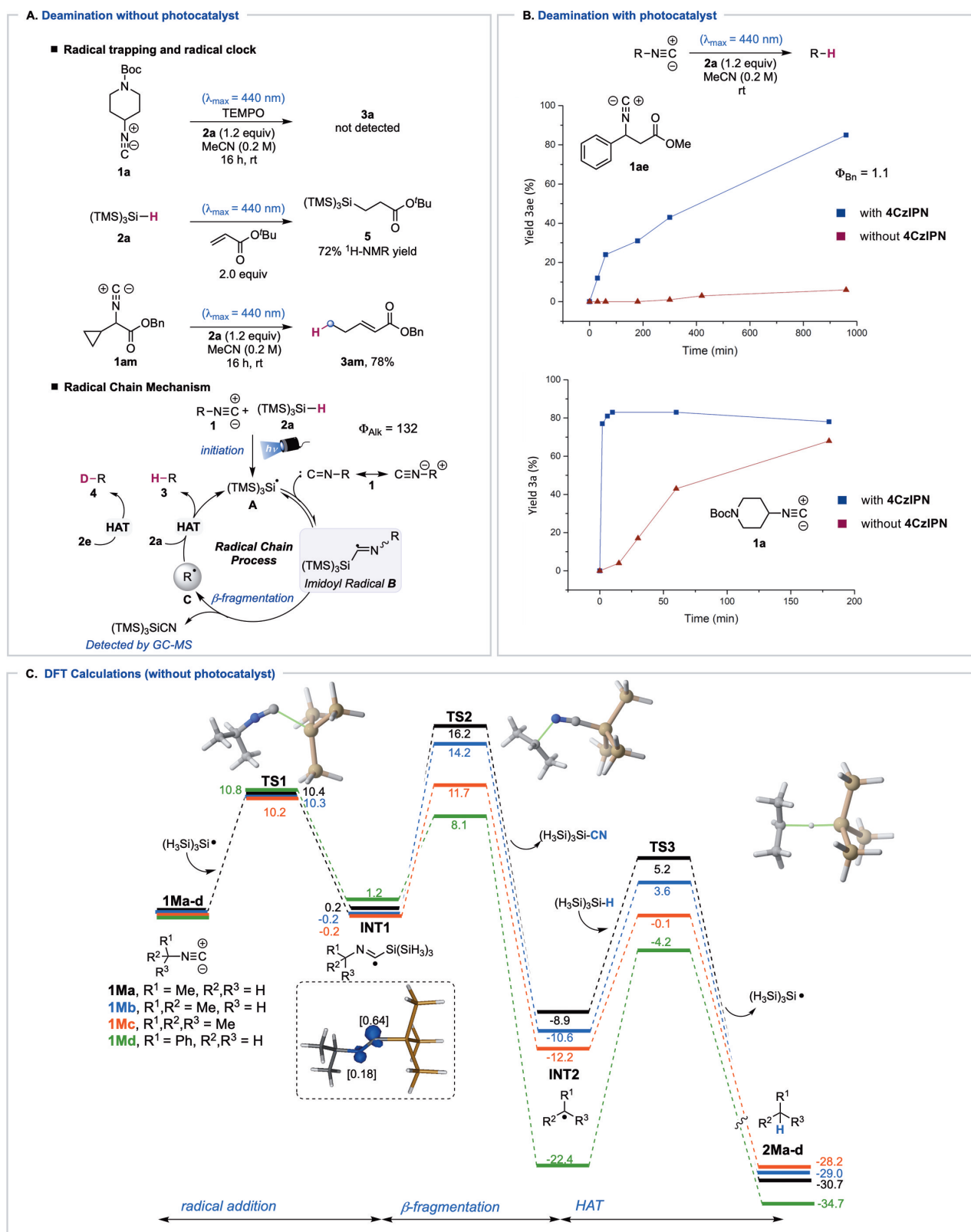
Figure 1. Mechanistic studies and DFT calculations (relative free energies are given in kcal/mol; all data have been computed at the PCM(acetonitrile)-M06-2X/def2-TZVP//PCM(acetonitrile)-M06-X/def2-SVP level).
