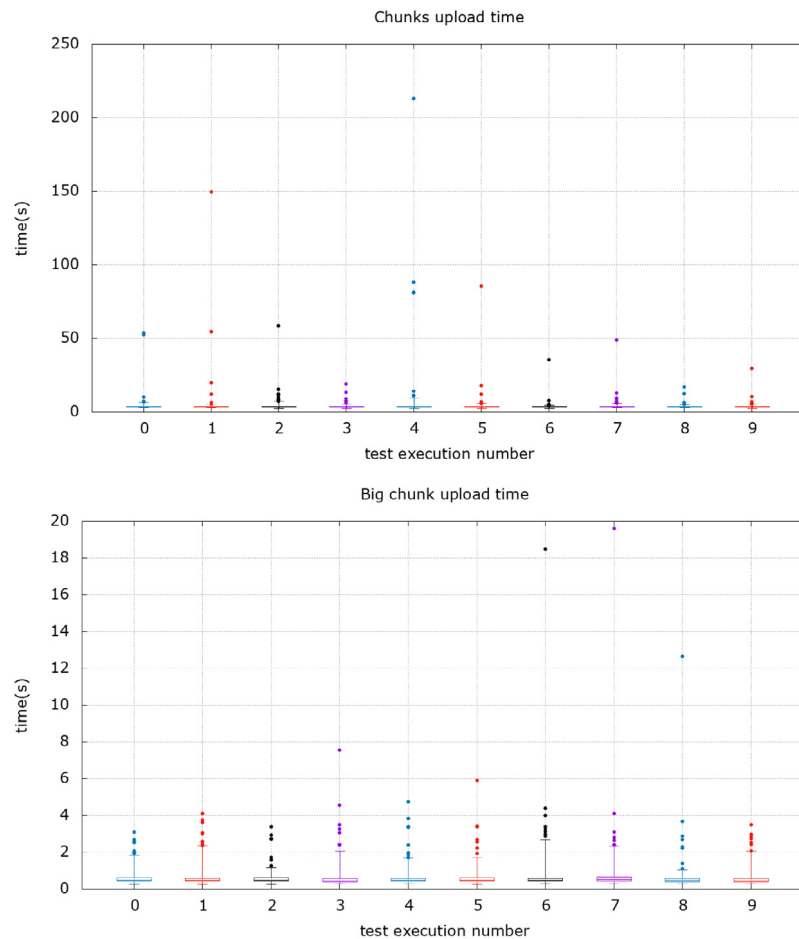
Fig. 9. Network test using 400 Lambda invocations with 3008 MB and 40 chunks. 10 test executions were performed. The plots show distributions of time required by Lambda invocations to conclude the small chunks upload step (up) and the “big chunk” upload step (down). Whiskers group the 98% of data. Coloured lines are only included for convenience. (For interpretation of the references to colour in this figure legend, the reader is referred to the web version of this article.)
