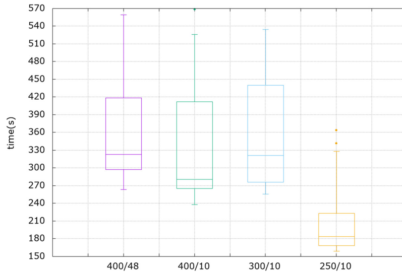
Fig. 5. Execution times distribution for “Aggregate 2a”. The x axis indicate the number of mappers and reducers used, using the format N_{mappers}/N_{reducers} . The number of executions done for each test are, respectively, 6, 10, 5, 20. Whiskers group the 90% of the data points.
