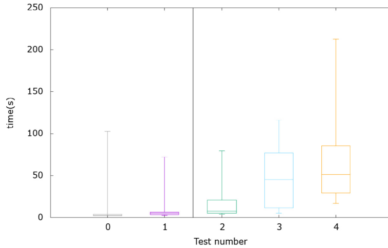
Fig. 12. Network performance assessment for Lambda function with 3008 MB. Represented tests use 20 and 40 chunks in the left and right of the vertical line, respectively. The number of simultaneous invocations is, in order, 20, 100, 100, 200 and 400. Plots show the distribution of required time, by the slowest invocation, to upload the corresponding number of chunks.
