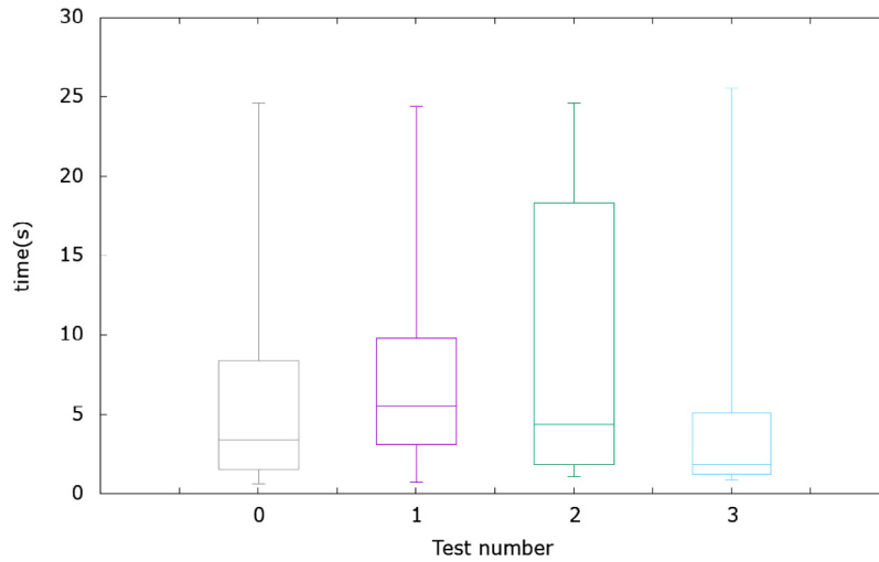
Fig. 13. Network test using 100, 200, 300 and 400 Lambda simultaneous invocations with 3008 MB and a single chunk. Plot shows distribution of required time, by the slowest invocation, to upload 1 chunk. Each test has been repeated 20 times.
