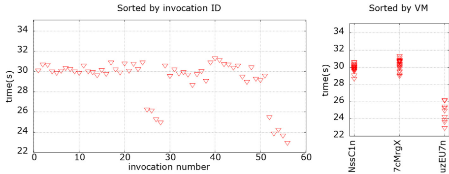
Fig. 6. Execution time distribution with 56 invocations of test Lambda function with 128 MB of memory. Invocations sorted by ID (left) and grouped by virtual machine identifier (right).
