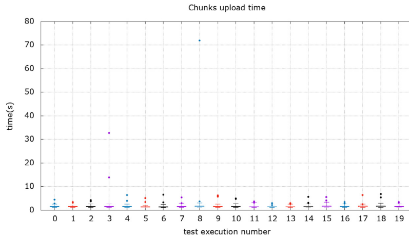
Fig. 10. Network test using 100 Lambda invocations with 3008 MB and 20 chunks. 20 test executions have been performed for this test. Plots show distributions of time required by invocations to conclude the small chunks upload step. Whiskers group the 98% of data.
