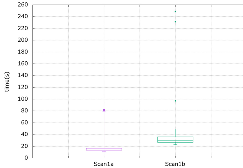
Fig. 2. Execution times distribution for Scan 1a and Scan 1b . Whiskers group the 90% of the data points. For Scan 1a , the execution times interval is, in seconds, [10.699, 81.874], with a mean value of 13.653 s. In the same way, the interval of Scan 1b is [22.758, 248.612] with a mean value of 29.635 s.
