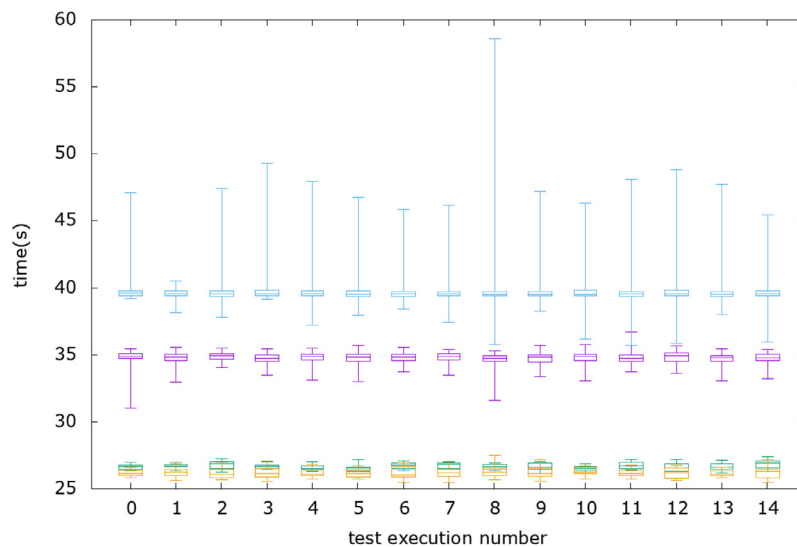
Fig. 8. Distribution of execution times for Lambda test invocations grouped by CPU model for each test execution. 200 invocations with 1216 MB have been used in this test. Each colour corresponds to one CPU model, Intel(R)-Xeon(R)-CPU-E5-2666-v3-@-2.90 GHz (purple), Intel(R)-Xeon(R)-CPU-E5-2676-v3-@-2.40 GHz (green), Intel(R)-Xeon(R)-CPU-E5-2680-v2-@-2.80 GHz (blue), Intel(R)-Xeon(R)-CPU-E5-2686-v4-@-2.30 GHz (yellow). (For interpretation of the references to colour in this figure legend, the reader is referred to the web version of this article.)
