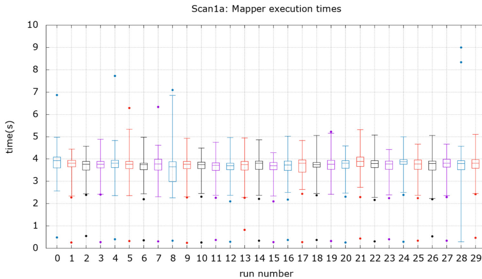
Fig. 3. Mapper execution times distribution for the “Scan 1a” query. Whiskers group 98% of total data points. Coloured lines are only included for the convenience of the reader. (For interpretation of the references to colour in this figure legend, the reader is referred to the web version of this article.)
