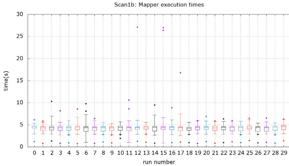
Fig. 4. Mapper execution times distribution for the “Scan 1b” query. Whiskers group 98% of total data points. Coloured lines are only included for the convenience of the reader. (For interpretation of the references to colour in this figure legend, the reader is referred to the web version of this article.)
