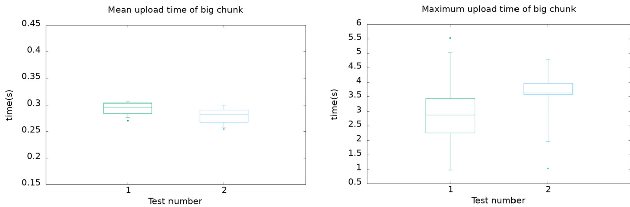
Fig. 15. Distributions of mean upload time (left) and maximum upload time (right) of big chunk step for test executions of each test. Each test has performed 10 executions with 100 Lambda invocations each one and 20 chunks. Whiskers include the 90% of all data so, one test execution is shown as a point.
