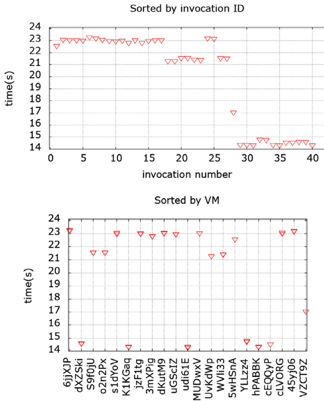
Fig. 7. Test with 40 invocations of test Lambda function with 1216 MB of memory. Invocations sorted by ID (up) and grouped by virtual machine identifier (down).
