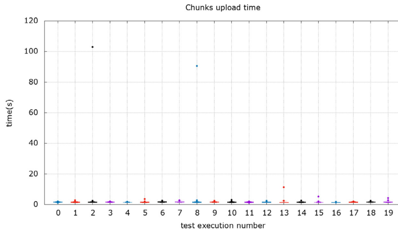
Fig. 11. Network test using 20 Lambda invocations with 3008 MB and 20 chunks. 20 test executions have been performed for this test. Plots show distributions of time required by invocations to conclude the small chunks upload step. Whiskers group the 90% of data.
