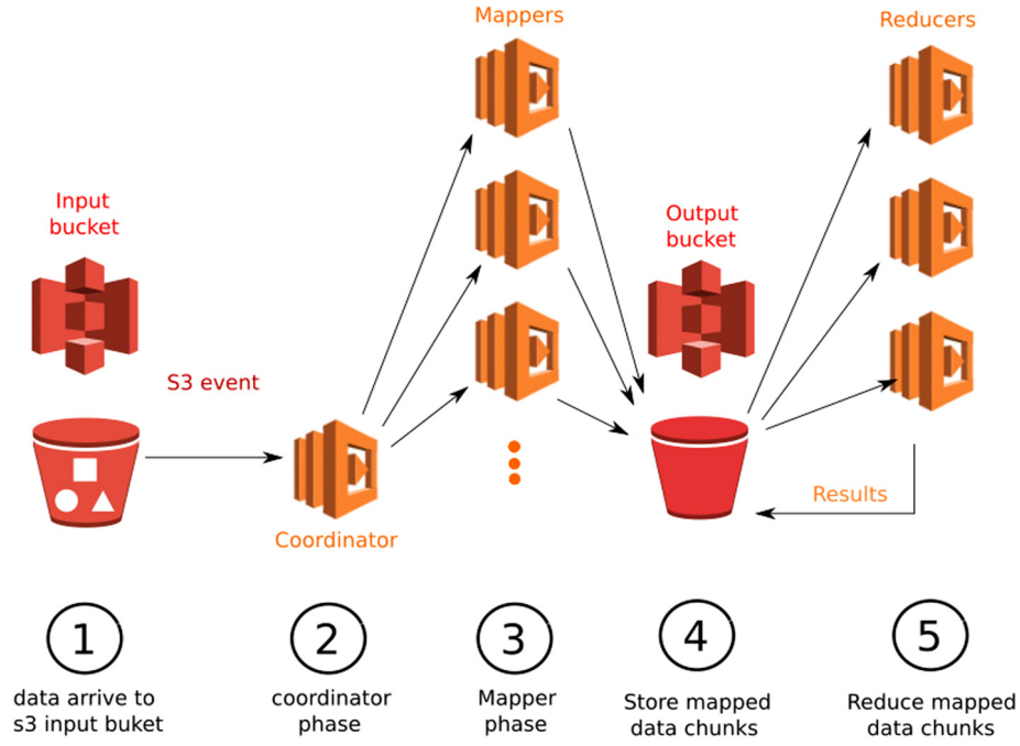
Fig. 1. Architecture of MARLA to support MapReduce on AWS Lambda.
