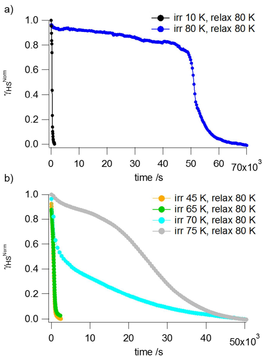
Evolution of the normalized photo-induced HS fraction as a function of time at 80K for the HS \rightarrow LS 1 relaxation after irradiation of the LS 1 phase at various temperatures. a) optical spectroscopy data b) magnetic data. All the experiments start from a quantitative population of the HS state by irradiation at the indicated temperature followed by a relaxation at 80 K.
