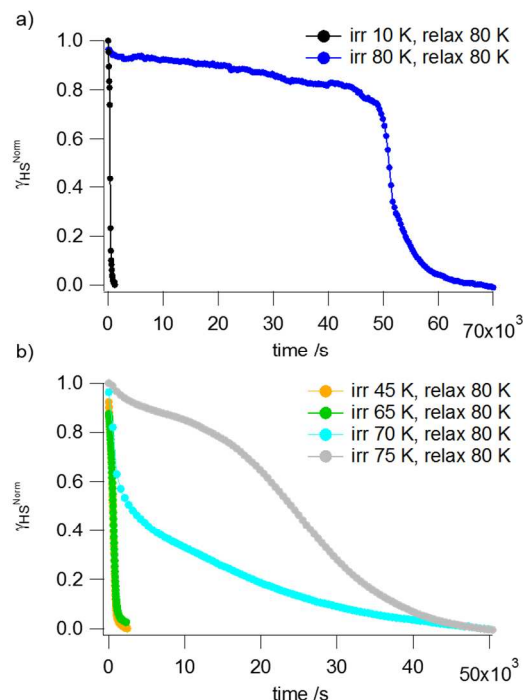
Figure 2. Evolution of the normalized photo-induced HS fraction as a function of time at 80K for the HS \rightarrow LS 1 relaxation after irradiation of the LS 1 phase at various temperatures. a) optical spectroscopy data b) magnetic data. All the experiments start from a quantitative population of the HS state by irradiation at the indicated temperature followed by a relaxation at 80 K.
