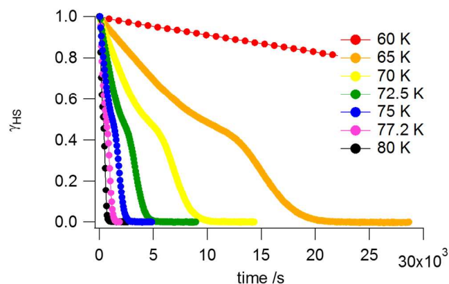
Figure 1. Evolution of the normalized photo-induced HS fraction as a function of time at various temperatures for the HS \rightarrow LS 1 relaxation after irradiation of the LS 1 phase. All the experiments start from a quantitative population of the HS state at 10 K followed by a relaxation at the indicated temperature.
