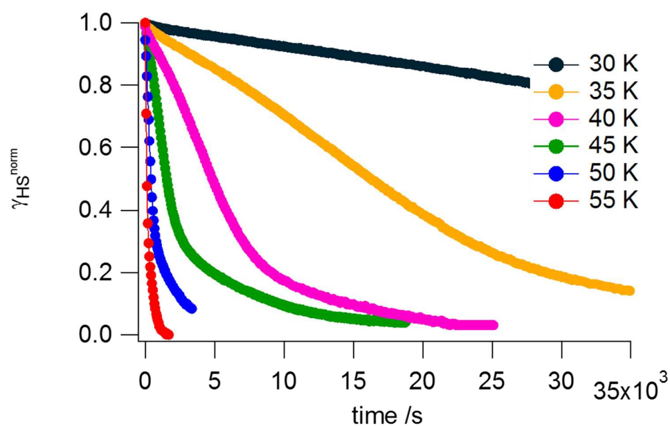
Figure 5. Evolution of the normalized photo-induced HS fraction as a function of time at various temperatures for the HS \rightarrow LS 2 relaxation after irradiation of the LS 2 phase. All the experiments start from a quantitative population of the HS state at 10 K followed by a relaxation at the indicated temperature.
