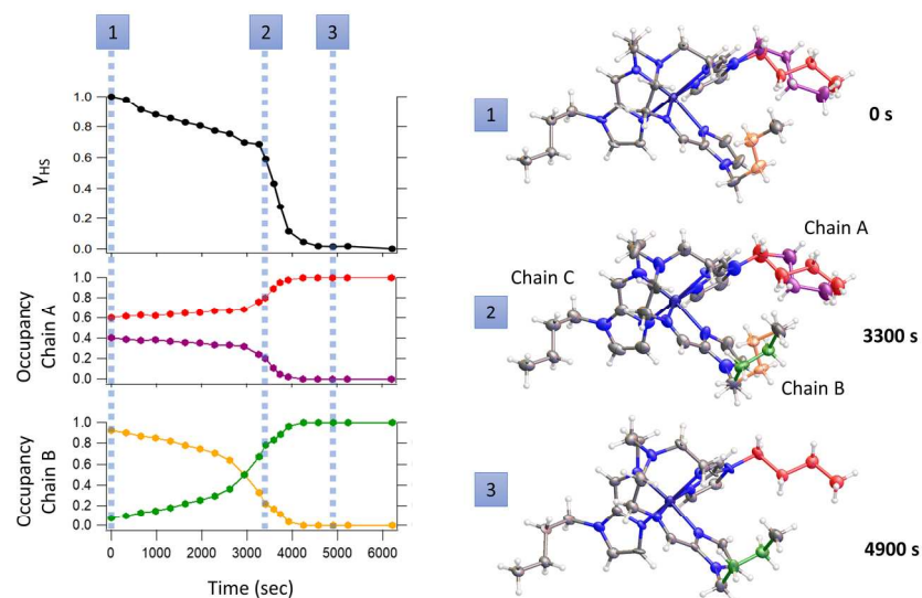
Figure 3. Relaxation curve obtained by single crystal X-ray diffraction using synchrotron radiation at 90 K after irradiation at the same temperature of the LS1 phase. The HS fraction curve (black) is derived from the crystallographic Fe-N distances. The structure of the complex is shown at three different relaxation times on this curve, with displacement ellipsoids depicted at 40 percent probability level. An order/disorder phase transition takes place in two different butyl groups of the ligand, chain A and B during the relaxation from HS11ir to LS1. For each chain, two different positions of the butyl group are observed, represented with different colors. The occupancy factor defines the proportion of the chain being in the given position. The evolutions with time of the occupancy factors for chain A and chain B are shown below the relaxation curve.
