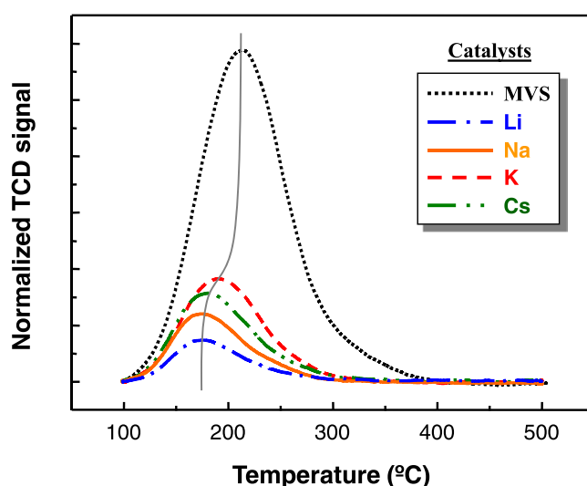
Fig. 2. TPD- \text{NH}_3 curves (normalized per mass unit) of alkali metal doped MoVSb mixed oxide catalysts ( \text{A}/\text{Mo} = 0.0025 ; \text{A} = \text{Li}, \text{Na}, \text{K} or \text{Cs} ) activated at 600 °C. Comparatively, the non-doped MoVSb mixed oxide catalyst (sample MVS) is also included. Detailed experiment conditions are in experimental section.
