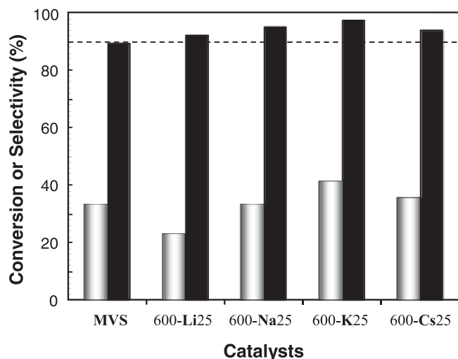
Fig. 5. Ethane conversion at a contact time, W/F, of 40 \text{ g}_{\text{cat}} \text{ h mol}_{\text{C}_2\text{H}_6}^{-1} (white bars), and selectivity to ethylene at ethane iso-conversion of 30 % (black bars), during ODH of ethane with alkali metal doped MoVSb mixed oxide catalysts (Alkali metal/Mo = 0.0025; activation at 600^\circ\text{C}/\text{N}_2 ). The non-doped MoVSb mixed oxide catalyst (MVS) is also included as reference. In all cases, data standard deviation was found below 2.1 % for conversion, and below 1.3 % for selectivity. Reaction conditions: Temperature = 400^\circ\text{C} ; Molar ratio of \text{C}_2\text{H}_6/\text{O}_2/\text{He} = 30/20/50 .
