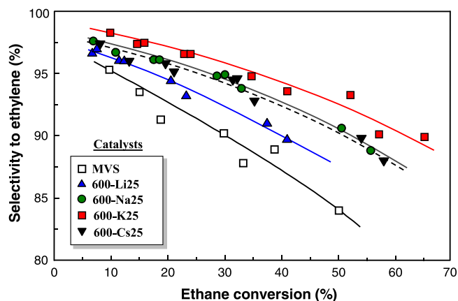
Fig. 7. Variation of the selectivity to ethylene with ethane conversion, obtained during ODH of ethane over alkali metal doped MoVSb mixed oxide catalysts (Li, Na, K or Cs) activated at 600^\circ\text{C}/\text{N}_2 . The non-doped MoVSb mixed oxide catalyst (MVS) is also included as reference. Reaction conditions: Temperature = 400^\circ\text{C} ; \text{C}_2\text{H}_6/\text{O}_2/\text{He} molar ratio of 30/20/50.
