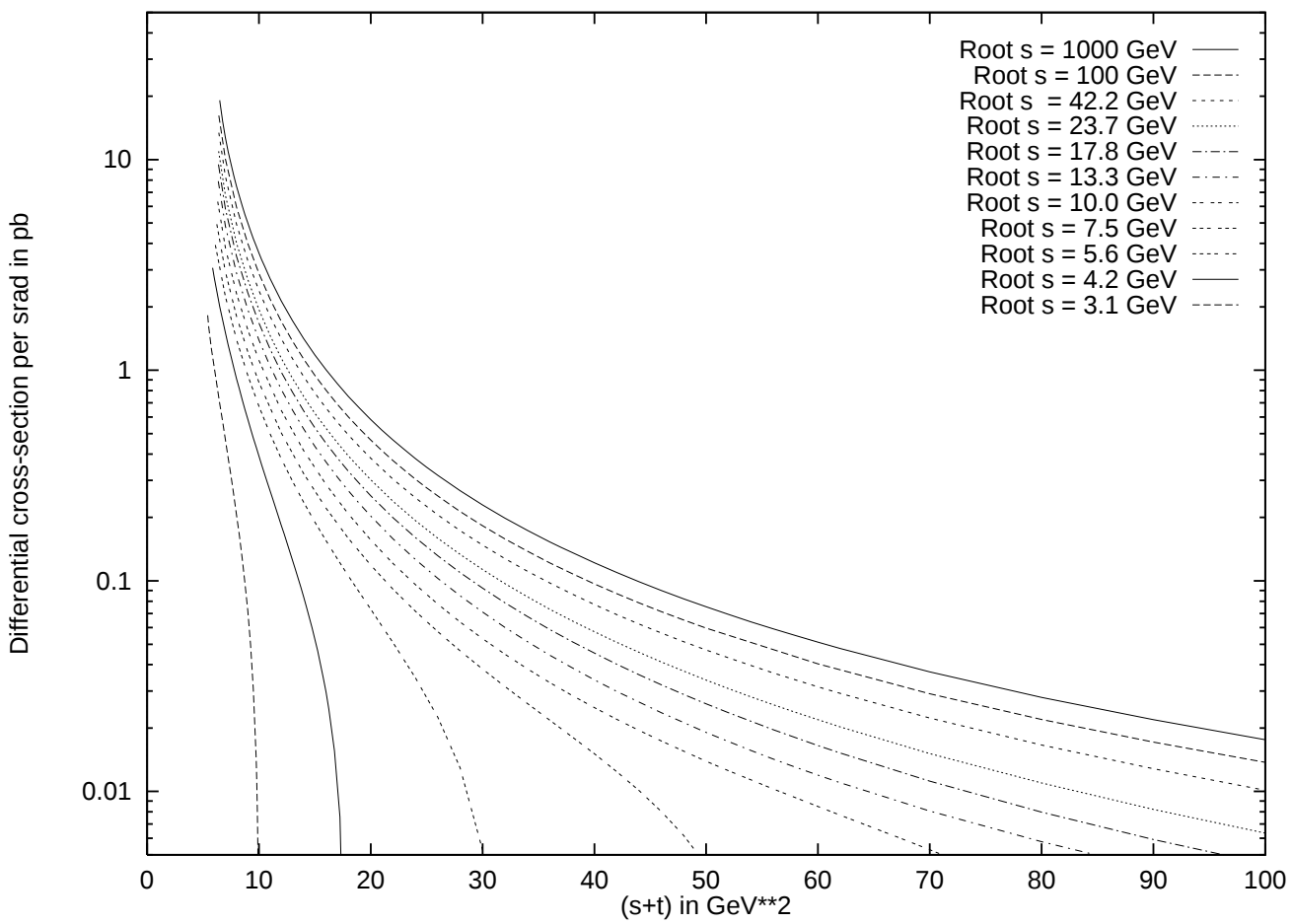
Figure 6: Spin- and polarization-summed differential cross section d\sigma/d\Omega for the transmutation process \gamma\mu \longrightarrow \gamma\gamma .
