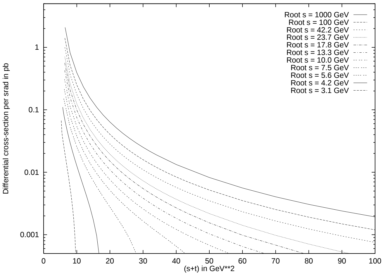
Figure 5: Spin- and polarization-summed differential cross section d\sigma/d\Omega for the transmutation process \gamma e \rightarrow \gamma T .
