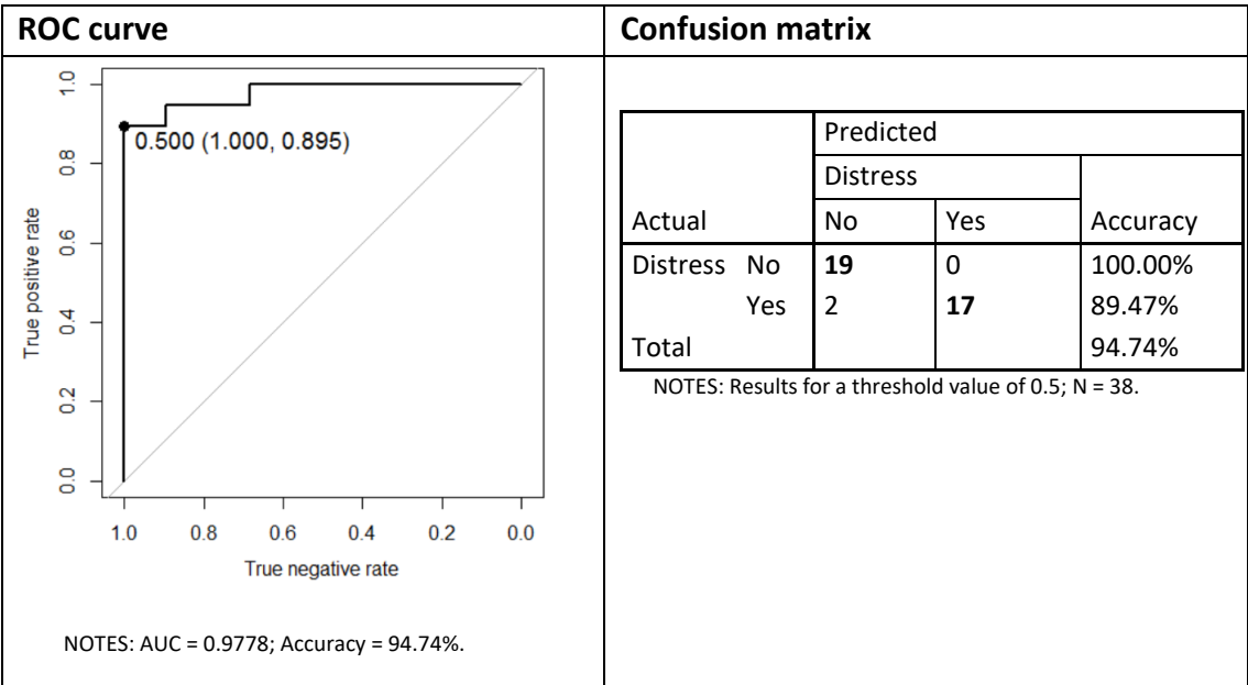
Fig. 8. Extreme gradient boosting performance for test dataset
