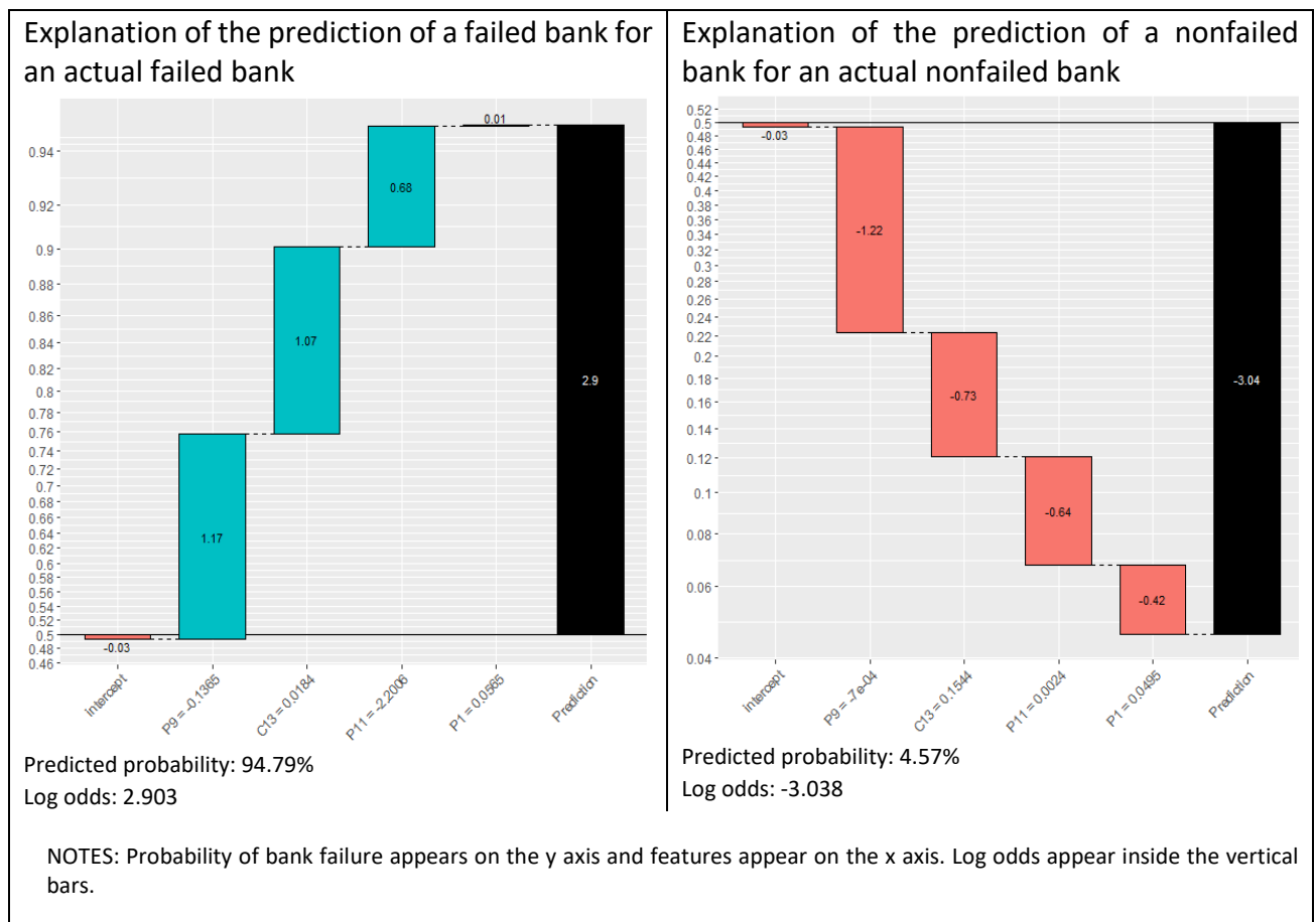
Fig. 16: Extreme gradient boosting prediction: Explanation of bank failure for two cases
