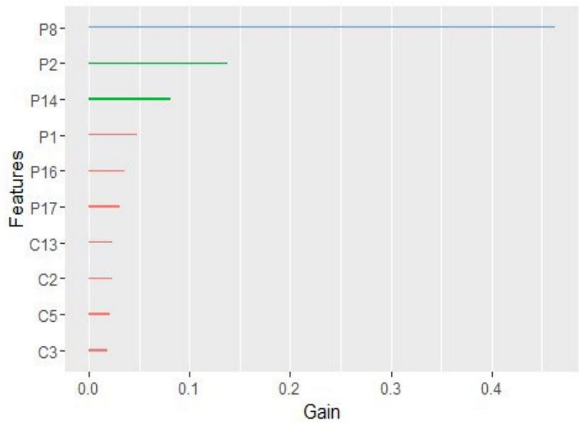
Fig. 11: Extreme gradient boosting performance for test data two years before failure
