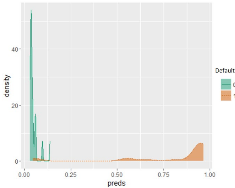
Fig. 9: Density plot of bank failure probability prediction for test dataset
