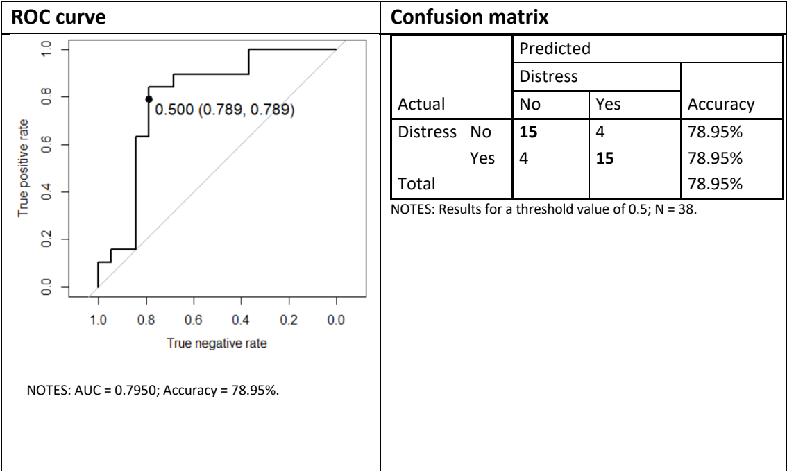
Fig. 13. Extreme gradient boosting performance for test data three years before failure
