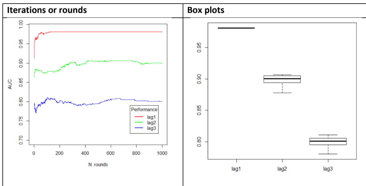
Fig. 14. 10-fold cross-validation AUC (ROC) performance distributions
