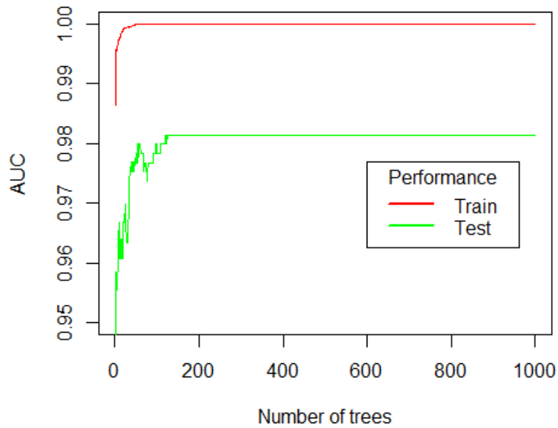
Fig. 5: Model 3: Training and test curves of AUC
