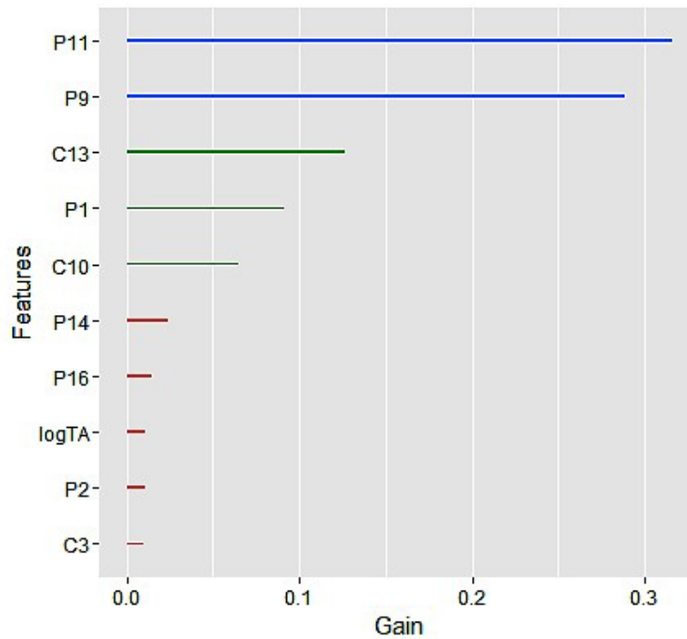
Fig. 6: Most important variables or features
