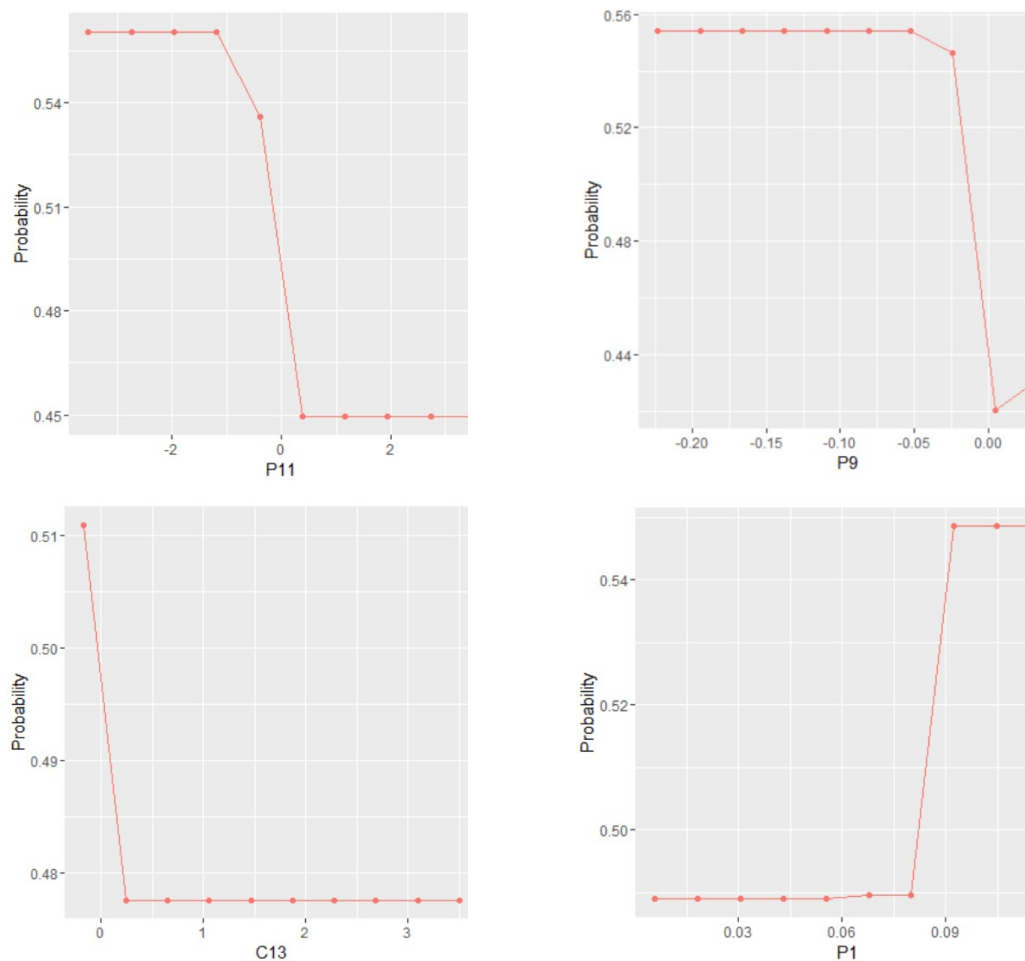
Fig. 7: Partial dependence plots for the four most influential variables
