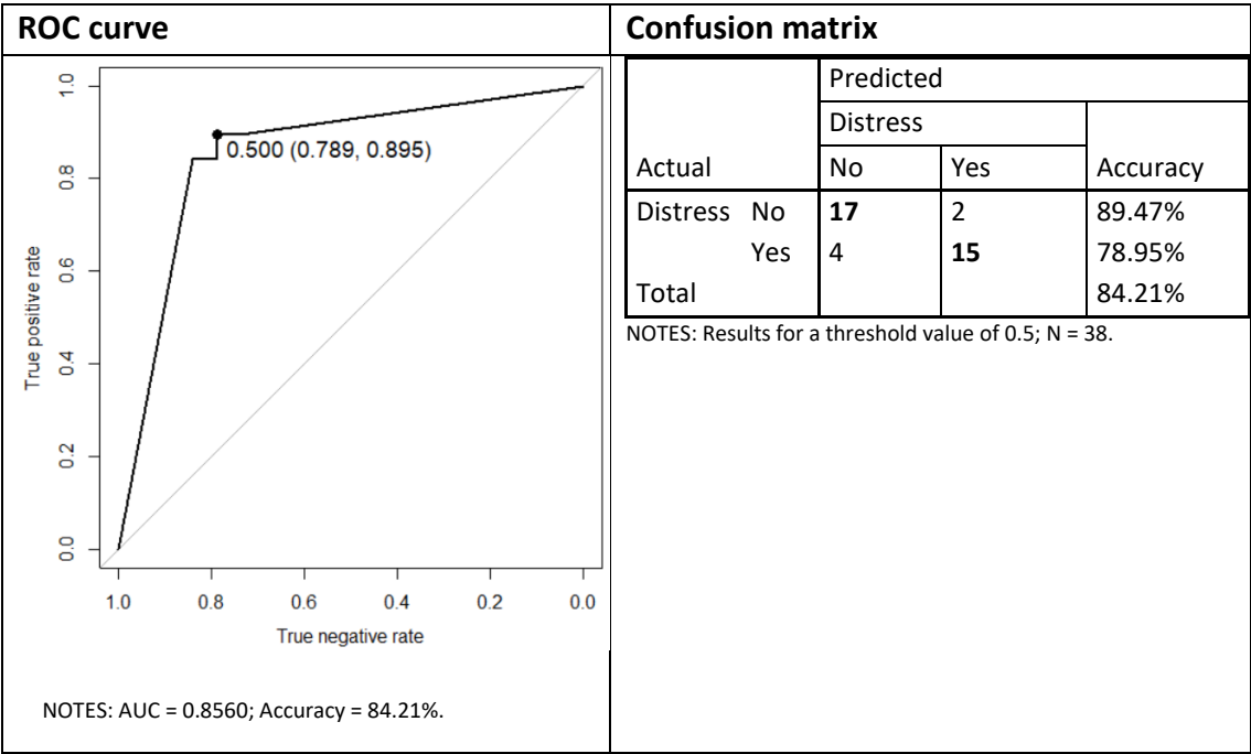
Fig. 17: Logistic regression performance for the test dataset
