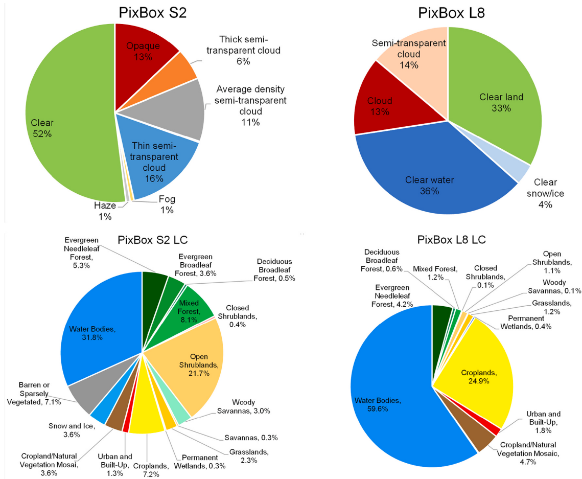
Fig. 6. Distribution of labeled pixels and land cover classes in the PiBoX dataset.
