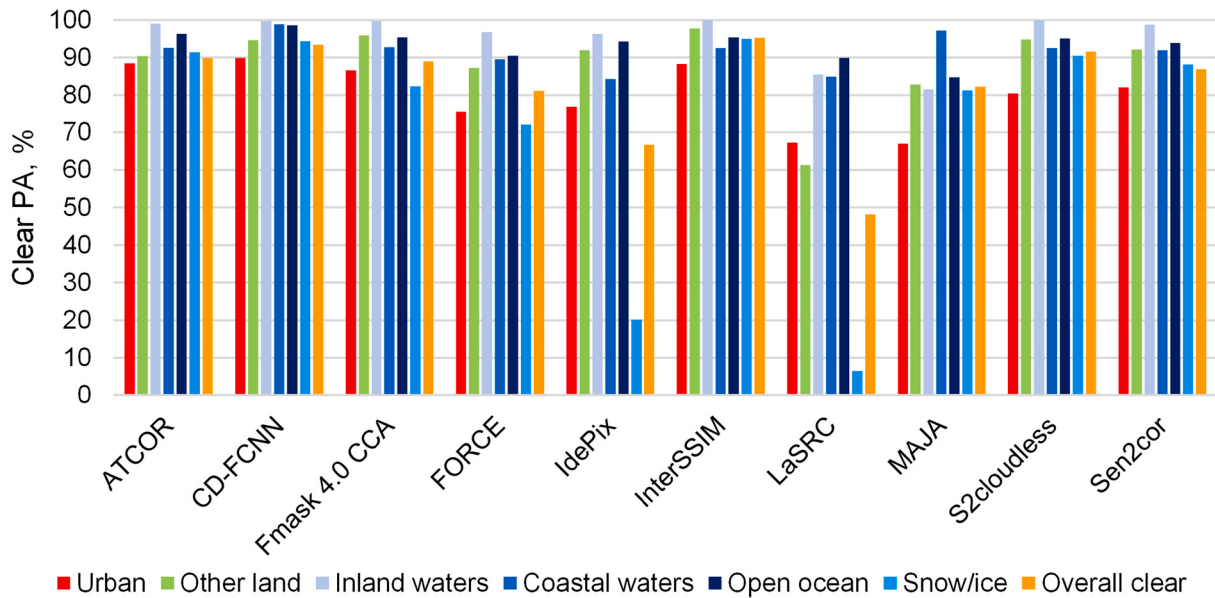
Fig. 14. Performance of algorithms in terms of clear producer's accuracy over the non-cloudy regions depending on the land cover types in the PiBox S2 dataset.
