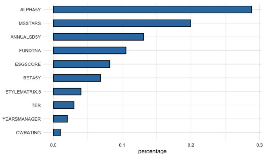
Fig. 4 Variable importance. XGBoost model
