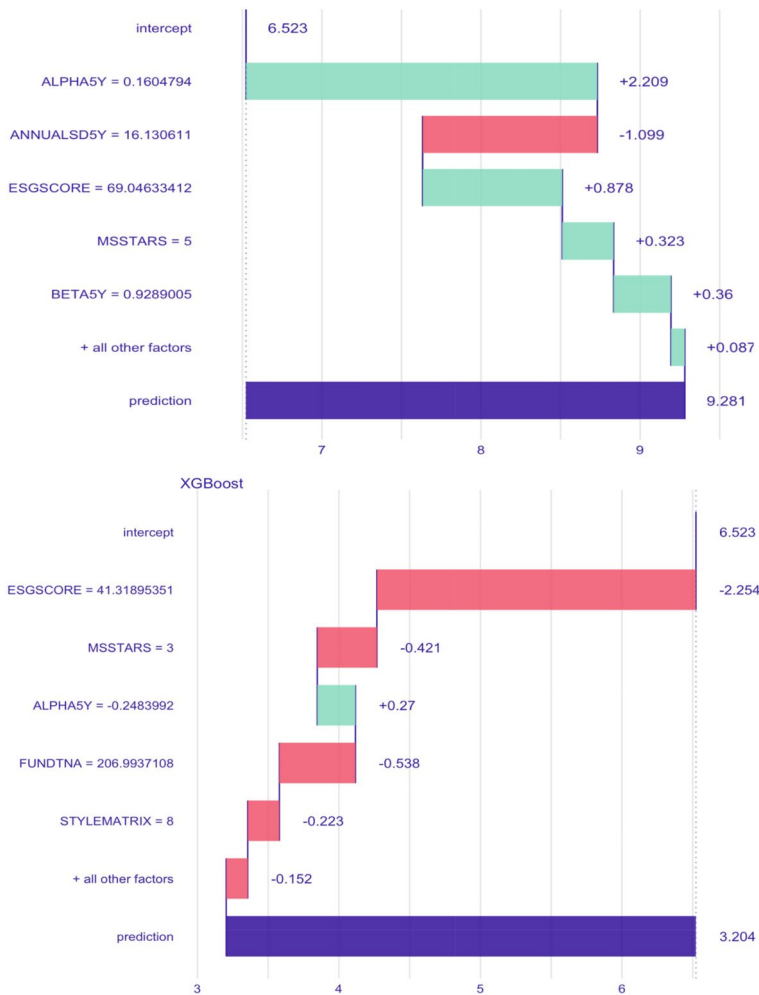
Fig. A1 Break-down plots for two observations from the test set. Notes: The upper observation has a high predicted value, which is higher than the average prediction. This suggests that ESG has a positive effect on the predicted fund return, which is included in all other factors. On the other hand, the lower observation has a predicted value that is lower than the average, indicating that ESG has a negative effect on the predicted fund return. Funding Open Access funding provided thanks to the CRUE-CSIC agreement with Springer Nature.
