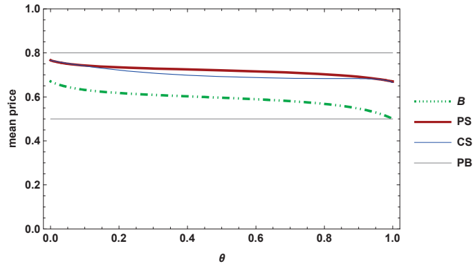
Figure 2 Mean price over the proportion of sophisticated traders, assuming \varepsilon = 0.025 in aggregate terms.
