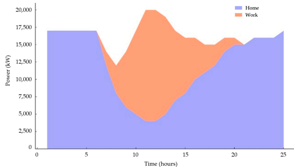
Figure 4. Estimation of V2G power flow during a typical workday.
