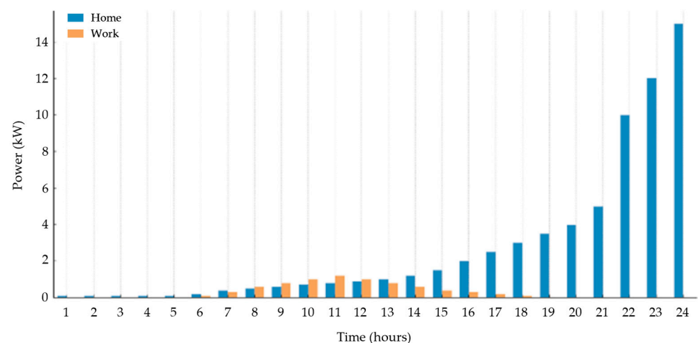
Figure 3. Estimation of G2V power flow in a working day.
