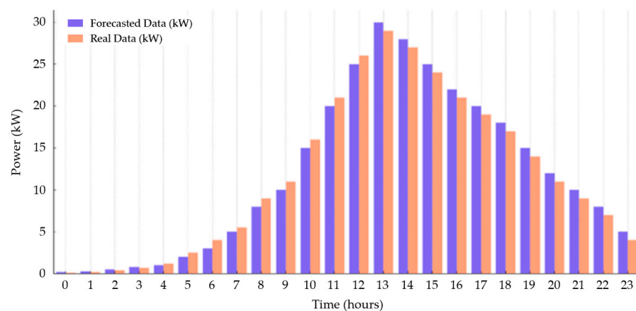
Figure 2. 24-h charging load profile: forecast accuracy assessment. Blue bars represent “Forecasted Data”, and orange bars represent “Real Data”.
