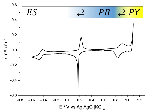
Figure 3. CV of PB in a 0.5 M KCl solution, pH=3.0 at 5 mV s -1
