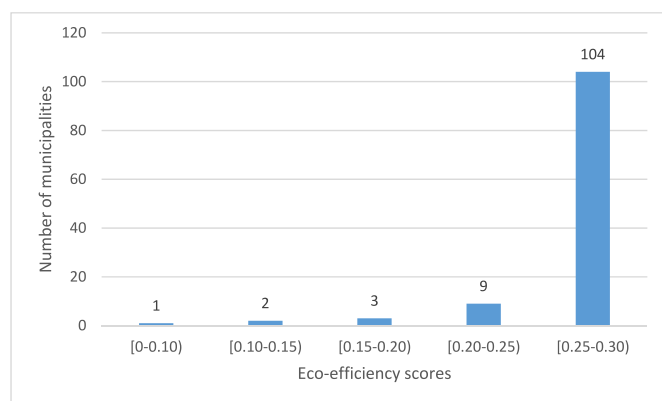
Fig. 1. Distribution of eco-efficiency scores across municipalities.
