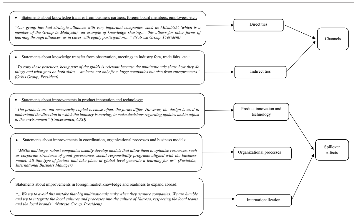
Figure 1. Data structure.
