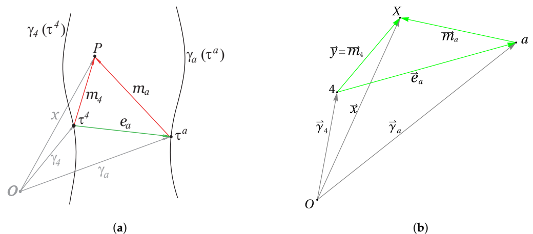
Figure 1. Configuration vectors in Minkowski space-time and in the 3-space orthogonal to u, E_\perp . (a) The fourth emitter \gamma_4 is taken as the reference emitter. Then, the position vector of the event P is m_4 . The relative positions e_a of the referred emitters \gamma_a are given by e_a = \gamma_a - \gamma_4 ( a = 1, 2, 3 ). This figure was taken from [7,8,26]. (b) In the 3-space orthogonal to u, E_\perp , taking the fourth emitter as the reference emitter, \vec{y} = \vec{m}_4 is the position vector of the user's location X . The relative positions \vec{e}_a of the referred emitters are given by \vec{e}_a = \vec{\gamma}_a - \vec{\gamma}_4 = \vec{m}_4 - \vec{m}_a ( a = 1, 2, 3 ).
