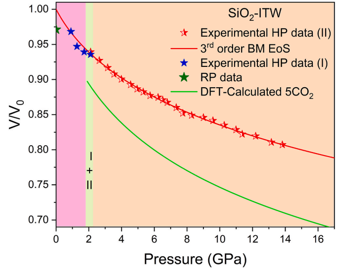
Fig. 9. P-V/ V_0 data per formula unit of CO 2 loaded pure-SiO 2 ITW zeolite. Blue (Phase-I) and red (Phase-II) star symbols refer to experimental data points. Error bars are smaller than symbol size. The red solid line represents the fit to the experimental data with a third-order Birch-Murnaghan EoS. The green solid line corresponds to DFT calculated data fitted with third-order Birch-Murnaghan EoS corresponding to 5 CO 2 molecules per unit cell.
