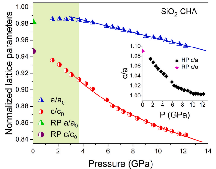
Fig. 4. Relative lattice parameters of CO 2 loaded pure-SiO 2 CHA framework under high pressure. Blue triangles represent the experimental data points of a/a_0 and the solid blue line is fitted data with second order isotherm BM EoS. Red circles show the experimental data points of c/c_0 and the solid red line is the fitted data of third order BM EoS. a_0 and c_0 values were obtained from the extrapolation of the fitting for P > 3.75 GPa data. Inset of the figure illustrates c/a ratios with pressure.
