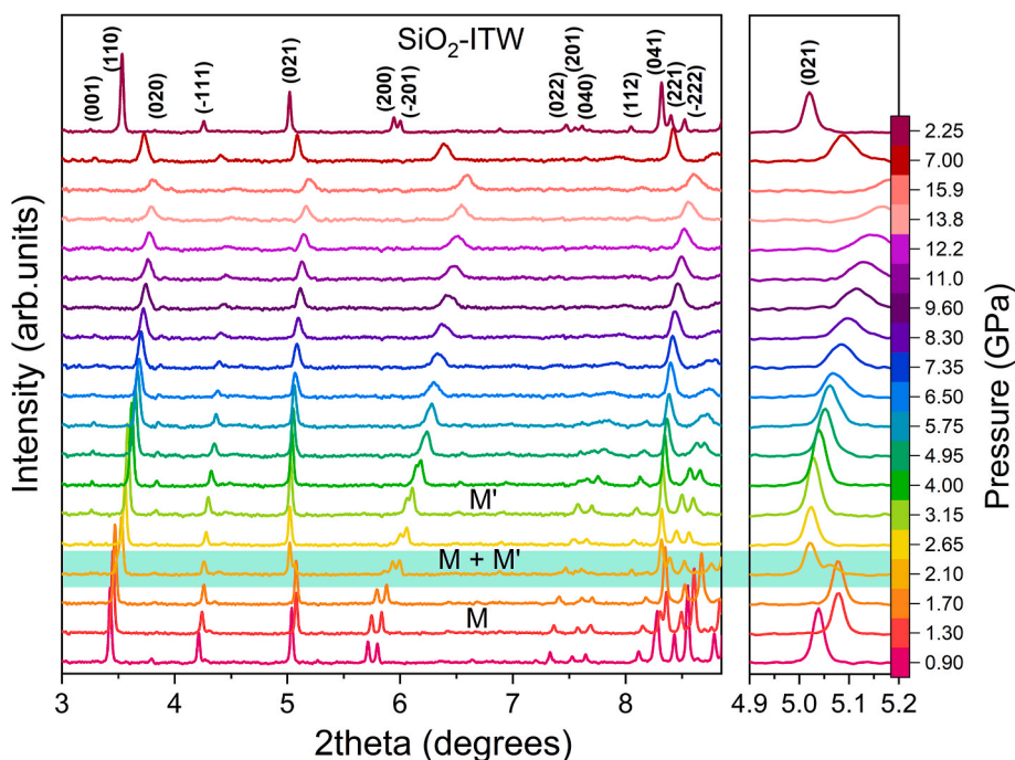
Fig. 7. Powder X-ray diffraction patterns of CO 2 -loaded pure-SiO 2 ITW zeolite up to 15.9 GPa ( \lambda = 0.4956 Å). As pressure increases, some peaks start to merge together and shift to the lower 2θ regions as the structure changes from monoclinic phase-I (M) to distorted monoclinic phase-II (M') at 2.1 GPa. For pressures above 5 GPa, the peaks broaden suggesting a pressure-induced loss of crystallinity. Nevertheless, there is no signature of pressure induced amorphization (PIA) up to the highest measured pressure. The measured pressure range covered in the experiment is displayed in the colour bar on the right-hand side.
