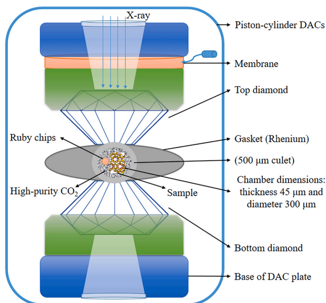
Fig. 1. Schematic diagram of the experimental set-up presenting membrane driven DACs having diamonds with 500 \mu\text{m} culets. The pressure chamber contains the zeolite sample, a small ruby chip as internal pressure gauge and high purity \text{CO}_2 as pressure transmitting medium (PTM), and it is sampled by the synchrotron X-rays.
