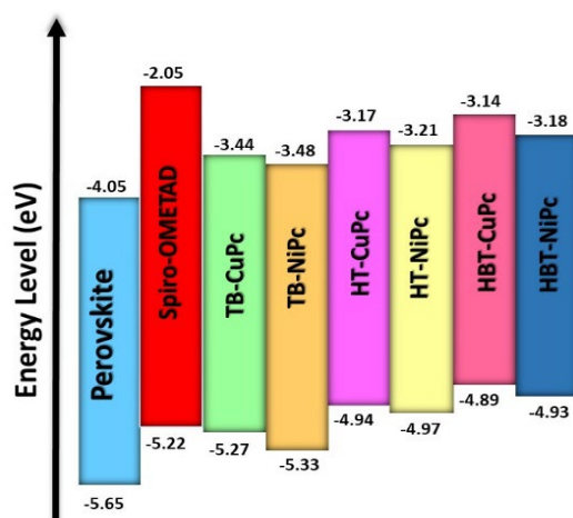
Figure 4. Energy band diagram of the MPc-based HTMs.
