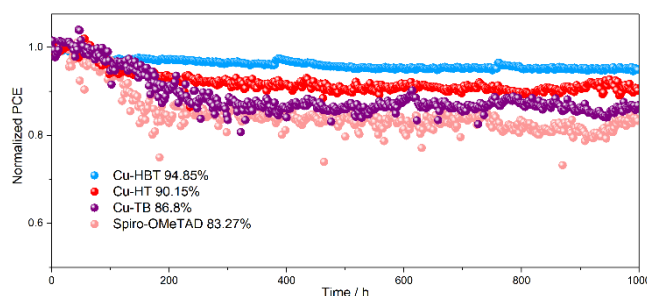
Figure 7. MPP stability of PSCs for CuPcs under the N 2 storage condition (25 °C)
