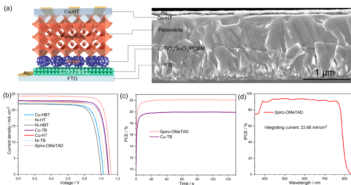
Figure 6. a) Illustration of the structure of ( n-i-p ) PSCs and the corresponding cross section-SEM of the device based on the HT-CuPc HTM. b) J-V curves of the devices using the different HTMs. c) The stabilized PCE under constant exposure of 1.5 AM light for spiro-
