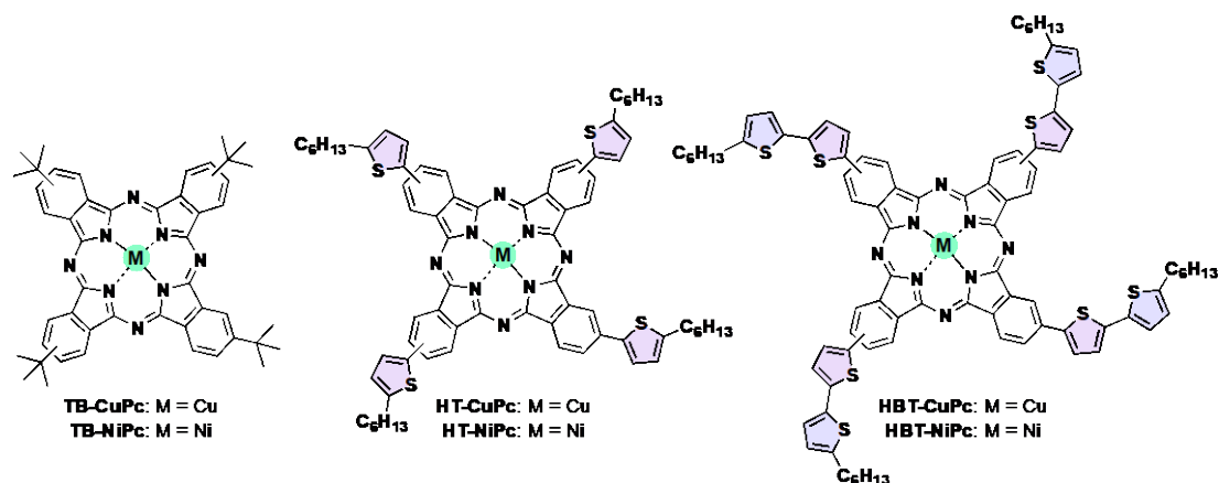
Figure 1. Molecular structures of TB-MPc, HT-MPc, and HBT-MPc, being M = Cu or Ni.
