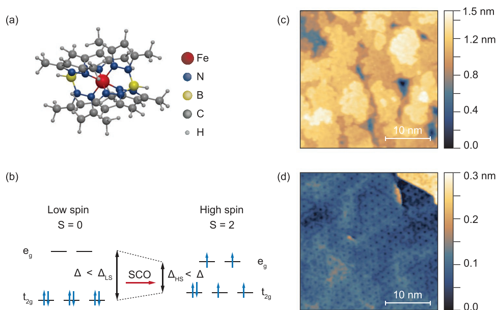
Figure 1. a) Schematic of a [Fe II (Pyrz) 2 ] molecule. The central Fe(II) ion is surrounded by six nitrogen atoms in octahedral symmetry. b) Simplified electronic configurations of the Fe(II) SCO molecule. The interplay between the ligand field strength ( \Delta_{LS} or \Delta_{HS} ) and the spin pairing energy ( \Delta ) determine the spin states. c,d) STM topography of Co film on Au(111) substrate before (c) and after (d) annealing process. The moiré pattern after annealing is indicative for a passivation by the Au overlayer. ( U = 1 V, I = 300 pA).
