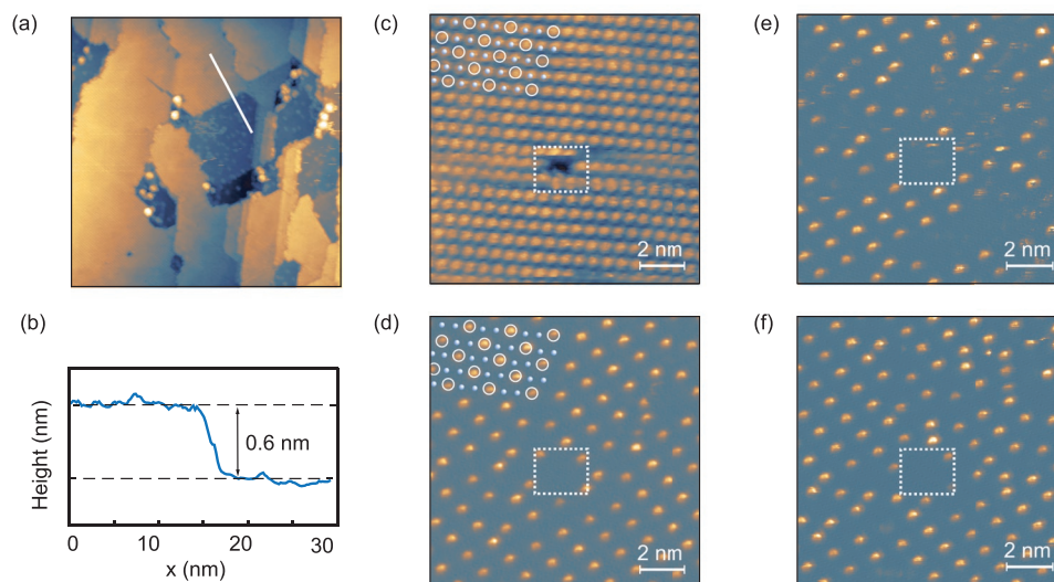
Figure 2. a) STM topography of self-assembled [\text{Fe}^{\text{II}}(\text{Pyrz})_2] molecules on Au-passivated Co/Au(111) ( U = -1 V, I = 50 pA, 85 \text{ nm} \times 85 \text{ nm} ). b) The line profile across the border of the molecular island as marked with white solid line in (a). c,d) STM images acquired at same scanning area in constant-current mode (c) ( U = -2 V, I = 50 pA) and constant-height mode (d) ( U = 300 mV, \langle I \rangle = 50 pA) showing patterns of different period. The former shows a full molecular crystal lattice, that is, both HS and LS molecules are visible, while the latter, under the specific voltage, only LS molecules appear as bright dots showing a mixed spin-state superstructure. The white circles (dots) mark the molecules in LS (HS) states and are the guide for the eyes. e) Constant-height images ( U = 300 mV, \langle I \rangle = 50 pA), acquired right after scanning the area at -2 V, showing a perturbed pattern. Some molecules fluctuate between HS and LS states. f) Constant-height image ( U = 300 mV, \langle I \rangle = 50 pA) acquired after 70 min after (e). The molecules relax to a more ordered pattern. Figure 2c–f is acquired at the same scanning area. The dashed rectangle is a mark of the defect for clarity. Image (d) was acquired after 3 h after (e).
