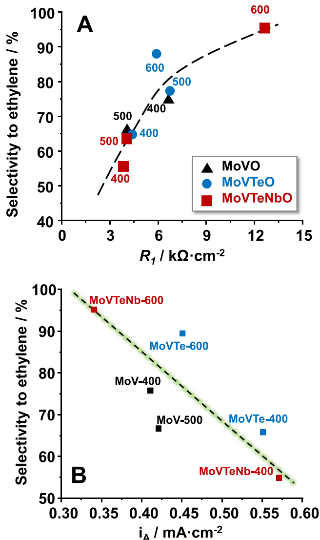
Fig. 8. Relationship between the selectivity to ethylene and the R_1 data (A) or the anodic current density, i_A , (B) for MoV-, MoVTe- and MoVTeNb-series catalysts calcined at 400, 500 and 600 °C. Note: Selectivity at 50 % ethane conversion and a reaction temperature of 390 °C.
