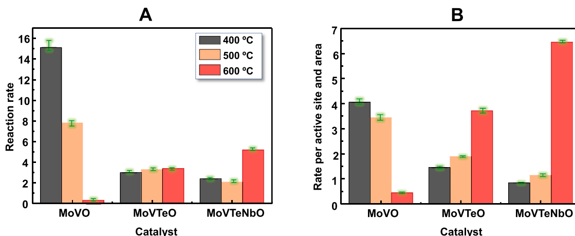
Fig. 4. Reaction rate of ethane conversion (A) and Reaction rate of ethane conversion per site and per area (B) of MoV-, MoVTeO- and MoVTeNbO-series, heat-treated at 400, 500 or 600 °C, during the ethane ODH. Reaction conditions: 390 °C and C 2 /O 2 /He: 5/5/90 molar ratio. Reaction rate as 10 3 mol C 2 H 6 g cat -1 h -1 at ethane conversions below 10 %. Reaction rate per active site and area as 10 3 mol C 2 H 6 (100 %V) -1 m -2 h -1 at ethane conversions below 10 %. Green bars correspond to error bars.
