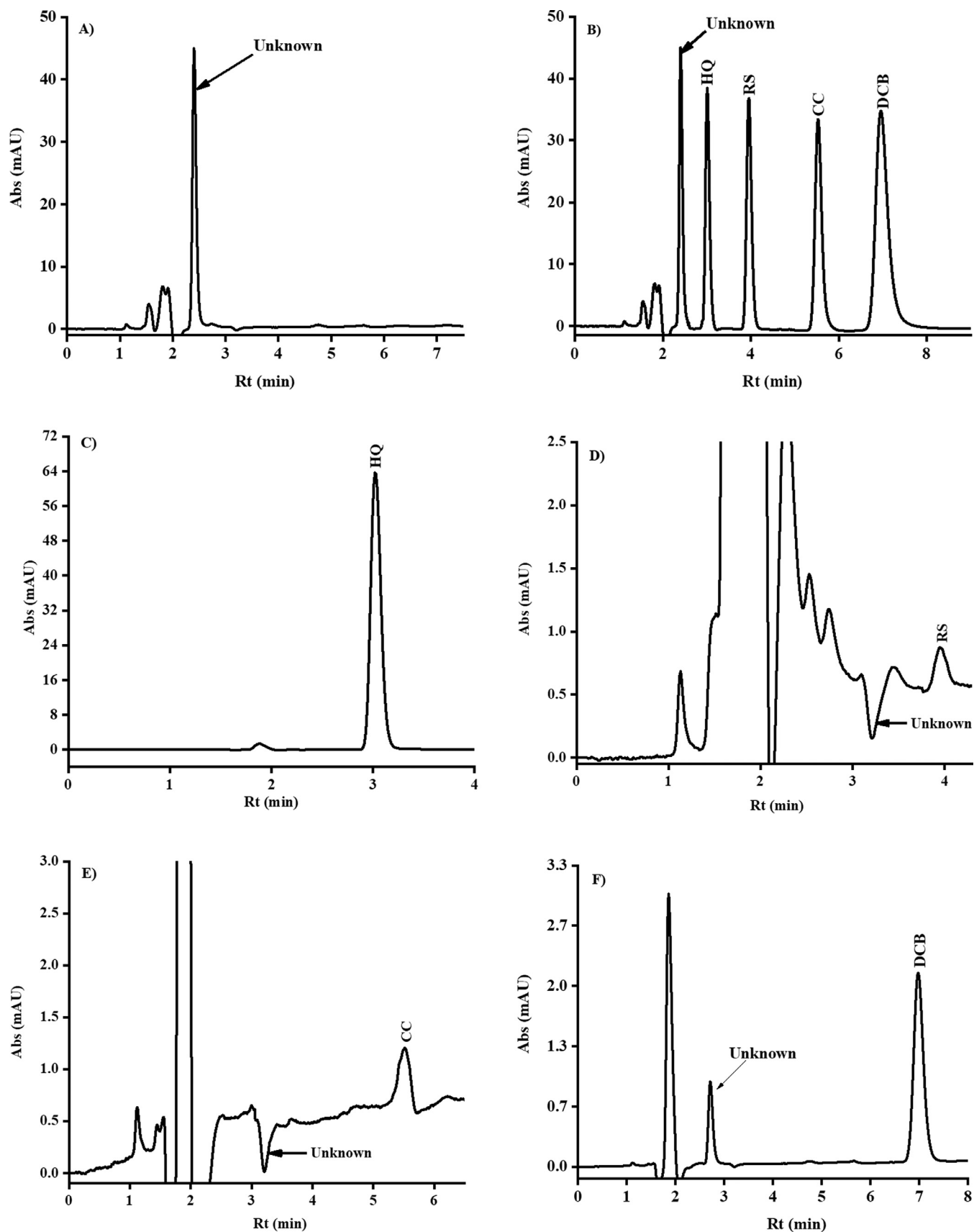
Fig. 2. Chromatograms obtained under the optimal conditions: (A) cream base (blank); (B) cream base (blank) spiked at 5 µg/100 mg (absorbance measured at 246 nm). Real obtained sample no.: 16. (C), 13. (D), 1. (E) and 8. (F), respectively.
