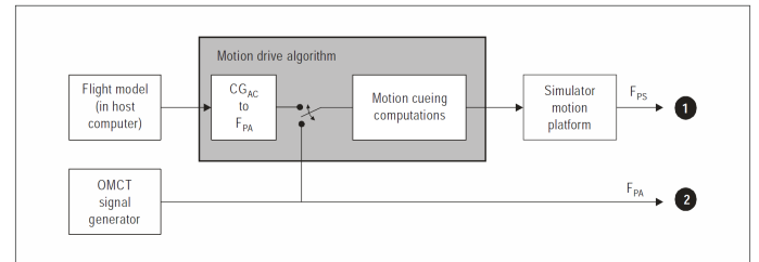
Fig. 4. OMCT working scheme (extracted from [52]).
