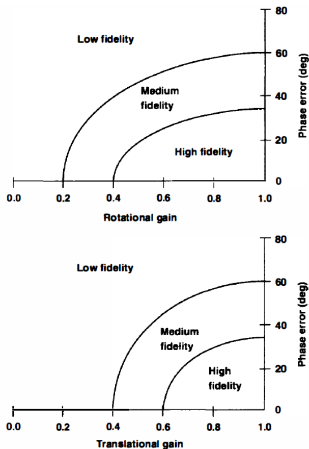
Fig. 2. Sinacori-Schroeder criterion and boundaries for the vertical axis (extracted from [49]).
