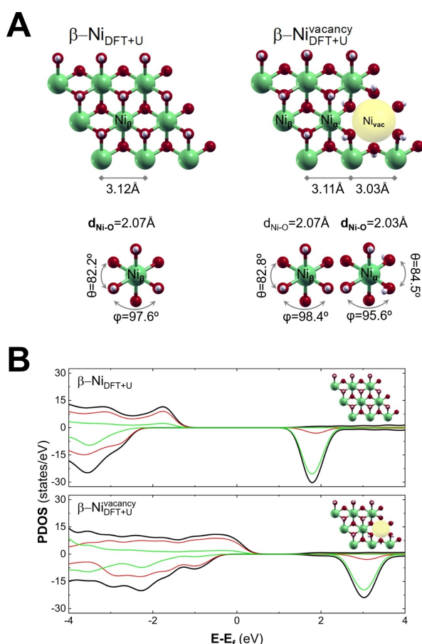
Figure 3. DFT + U simulations for a single layer of brucitic-like \text{Ni}(\text{OH})_2 structure ( \beta - \text{Ni}_{\text{DFT+U}} ) and the resulting one after the Ni-vacancies generation ( \beta - \text{Ni}_{\text{DFT+U}}^{\text{vacancy}} ). A) Relaxed structures for both supercell highlight that while \beta - \text{Ni} contains only one cationic environment ( \text{Ni}_\beta ), in the case of \beta - \text{Ni}^{\text{vacancy}} presence of two different Ni sites are observed: \text{Ni}_\alpha for the atom around the vacancy, and \text{Ni}_\beta for the other ones. Calculated structural parameters, such as Ni–O and Ni–Ni distances and angles for both supercells are shown. B) Total and Projected Density of States (PDOS) for a layer of \beta - \text{Ni}(\text{OH})_2 structure (upper panel) and the resulting one after the generation of Ni-vacancies (lower panel). Atoms are labelled according to Figure 1: H – white, O – red, Ni – green, Ni-vacancy – yellow.
