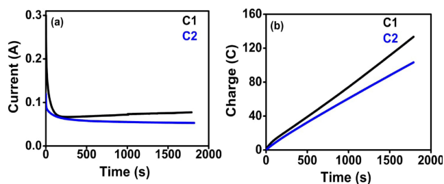
Figure 8. (a) CPE of C1 and C2 in 1.0 M KOH (pH \sim 11.6 ) solution, and (b) the subsequent \text{O}_2 evolution of C1 and C2 during the CPE.
