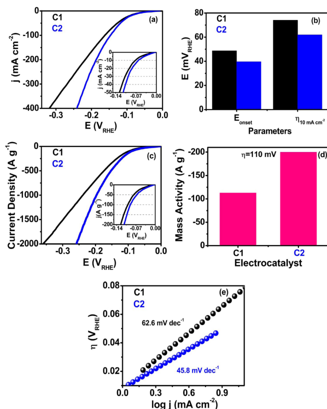
Figure 5. (a) HER polarization curves in 1.0 M KOH under 1600 rpm rotational speed (inset, LSV plot up to current density of -50 \text{ mA cm}^{-2} ), (b) bar diagram representing E_{\text{onset}} and \eta_{10} \text{ mA cm}^{-2} , (c) mass activity plots (inset, plot up to current density of -200 \text{ A g}^{-1} ), (d) bar diagram of mass activity at \eta = 110 \text{ mV} , and (e) the corresponding Tafel plots of both ECs.
