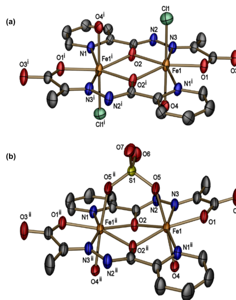
Figure 1. The structure of (a) C1 and (b) C2 with displacement ellipsoids drawn at 40% probability level. Hydrogen atoms are omitted for clarity. Only one orientation of the disordered \text{SO}_4^{2-} in C2 is shown. Symmetry codes: (i) 1-x, 1-y, 1-z ; (ii) 1-x, y, 0.5-z .
