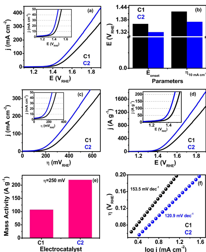
Figure 3. (a) OER polarization curves in 1 M KOH under 1600 rpm rotational speed (inset, LSV plot up to current density of 50 \text{mA cm}^{-2} ), (b) bar diagram representing E_{\text{onset}} and \eta_{10} \text{mA cm}^{-2} , (c) the current density vs. \eta plots (inset, LSV plot up to current density of 50 \text{mA cm}^{-2} ), (d) mass activity plots (inset, plot up to current density of 220 \text{A g}^{-1} ), (e) bar diagram of mass activity at \eta = 250 mV, and (f) OER Tafel plots of C1 and C2 .
