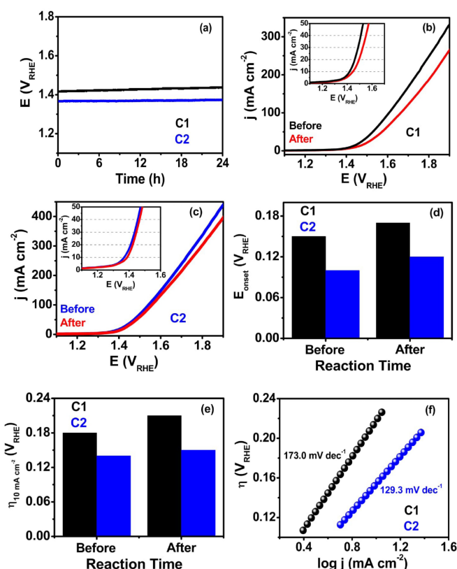
Figure 4. (a) Chronopotentiometric measurements of ECs at 10 \text{ mA cm}^{-2} for 24 h in 1 M KOH under 1600 rpm rotational speed; OER polarization curves in 1.0 M KOH under 1600 rpm rotational speed of (b) C1 and (c) C2 before and after 5000 cycles stability test (both insets, LSV plots up to current density of 50 \text{ mA cm}^{-2} ); Bar diagram of (d) \eta_{\text{onset}} and (e) \eta_{10} of before and after 5000 cycle's stability test; (f) OER Tafel plots after 24 h stability test.
