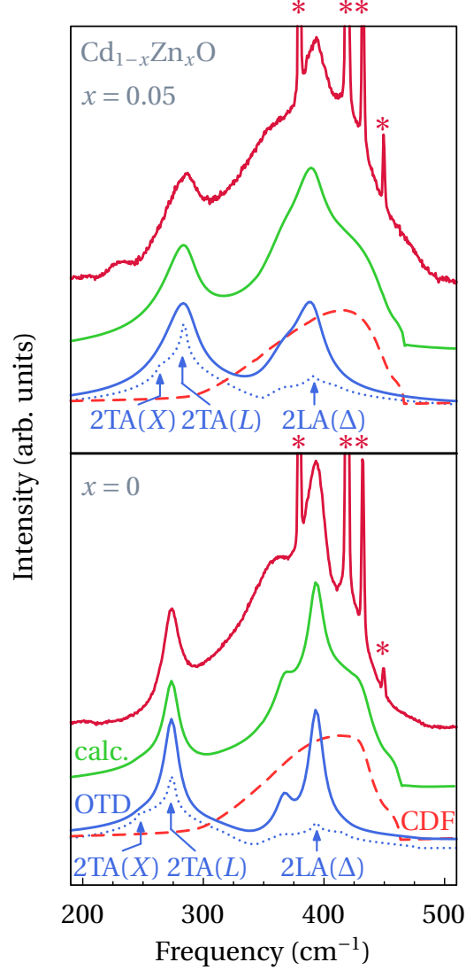
FIG. 1. Raman spectra of CdO and \text{Cd}_{0.95}\text{Zn}_{0.05}\text{O} at 80 K (top red curves in each panel) and the different contributions in the spectral region of the acoustic overtones. The dotted line is the phonon-overtone density of states. The peaks corresponding to the critical points in the PDOS ( L , X , and \Delta \sim \frac{2}{3}\bar{\Gamma}-\bar{X} ) are indicated by the arrows. The dashed line represents the charge-density-fluctuation (CDF) scattering and the blue curve corresponds to the overtone contribution (OTD) to the Raman spectra. The green curve (calc) is the calculated spectrum obtained by adding these two contributions. The peaks marked with asterisks correspond to the sapphire substrate.
