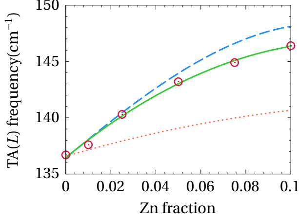
FIG. 6. Dependence of the TA(L) frequency on the alloy composition. Circles correspond to the halved frequency of the 2TA(L) feature in the Raman spectra (the solid line is a guide to the eye). The dashed line indicates the corresponding frequency of the NNN cation-sublattice model. The ab initio VCA calculations with averaged pseudopotentials are shown as a dotted line.
