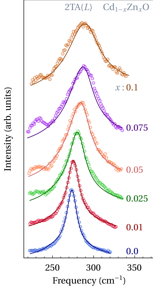
FIG. 5. Line-shape simulations of the 2TA(L) peak of \text{Cd}_{1-x}\text{Zn}_x\text{O} for 0 < x < 0.1 using the ICPA model (solid lines) compared with the 80 K Raman spectra (circles). For the sake of comparison, the spectra have been normalized to have the same peak intensity.
