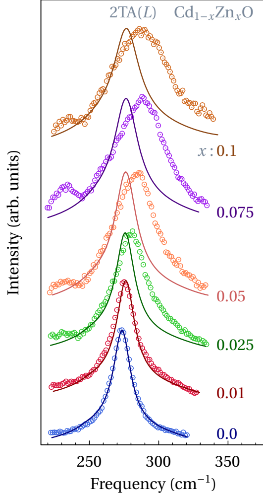
FIG. 3. Raman spectra of the 2TA(L) peak at 80 K of \text{Cd}_{1-x}\text{Zn}_x\text{O} for 0 < x < 0.1 after background subtraction (circles). The solid lines are the mass-disorder broadened line shapes as predicted by the CPA model.
