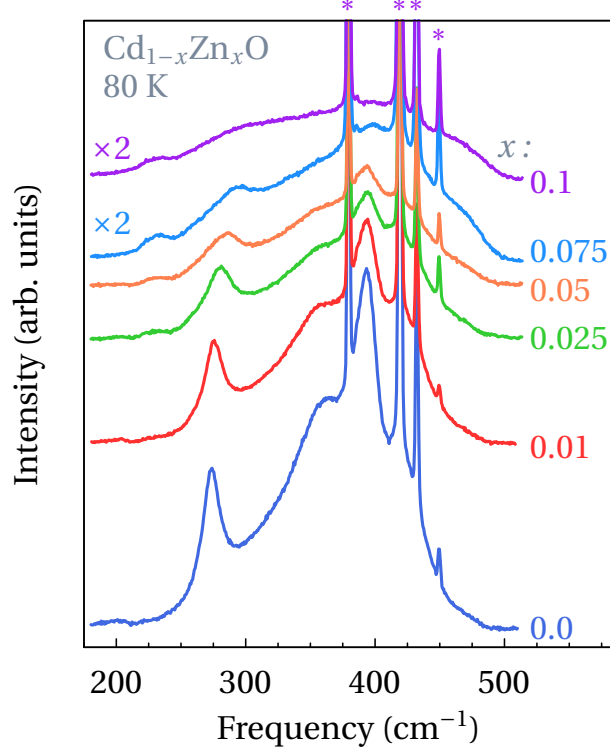
FIG. 2. Raman spectra of \text{Cd}_{1-x}\text{Zn}_x\text{O} alloy for increasing Zn fraction at 80 K in the spectral region of the acoustic overtones. The peaks marked with asterisks correspond to the sapphire substrate.
