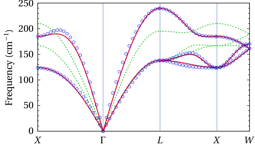
FIG. 4. Acoustic phonon dispersion of CdO along high-symmetry directions calculated in the next-nearest-neighbor approximation of the cation sublattice (solid lines), compared to full-crystal ab initio calculations (circles). The dotted lines display the results of the nearest-neighbor approximation.
