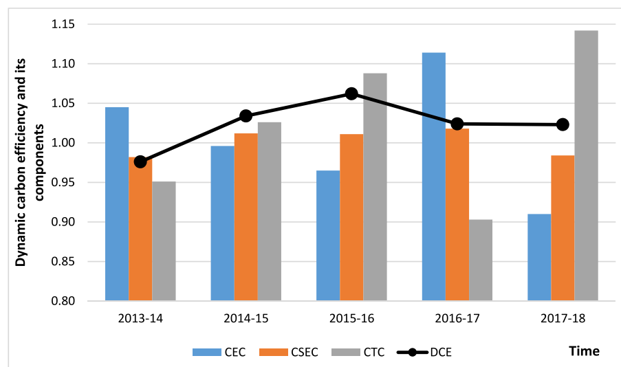
Fig. 4. Average dynamic carbon efficiency and drivers for English and Welsh water and sewerage companies (WaSCs).
