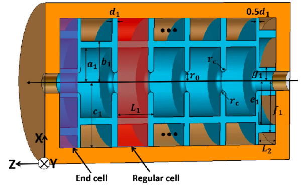
Fig. 1. Schematic of a DAA structure with its characteristic dimensions. Source: Figure extracted from [6].
