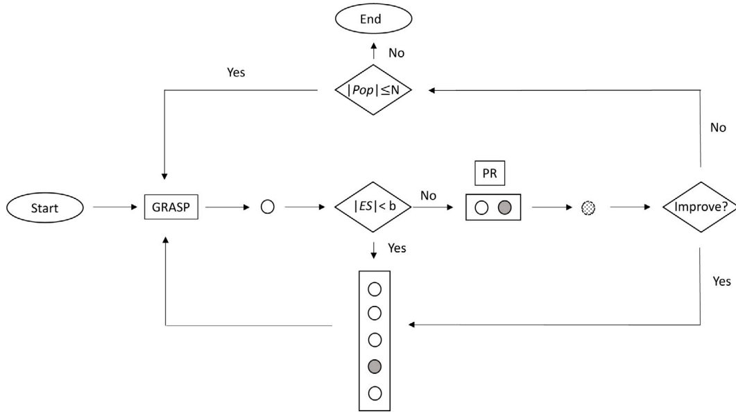
Fig. 3. Dynamic GRASP with PR.
