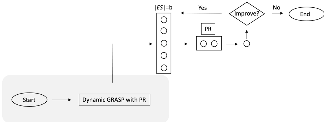
Fig. 4. GRASP with Evolutionary PR.
