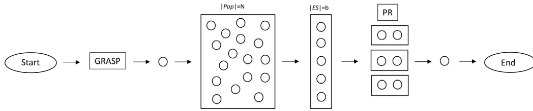
Fig. 2. Static GRASP with PR.
