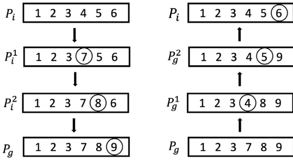
Fig. 5. Interior Path Relinking.
