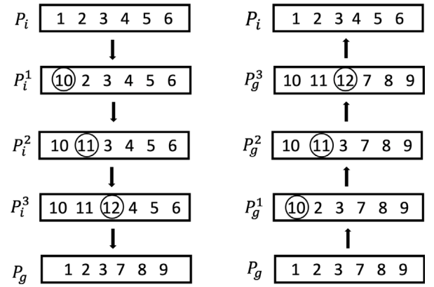
Fig. 6. Exterior Path Relinking.
