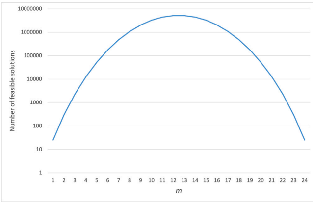
Fig. 1. Number of solutions, as a function of m = p + q in the x-axis, of an instance with n = 25 .
