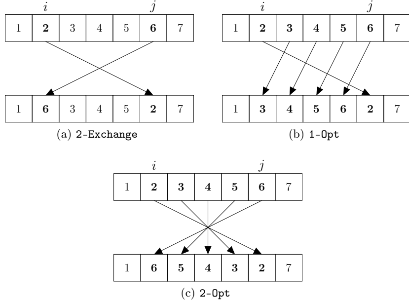
Figure 2: Examples of the different applications of local search procedures.
