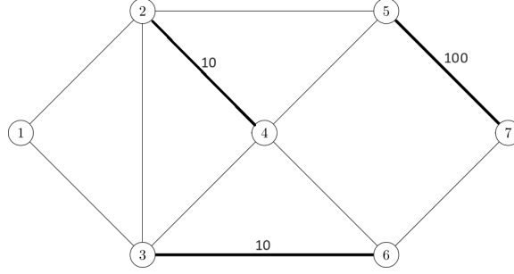
Figure 1: An example of a graph with seven nodes.
