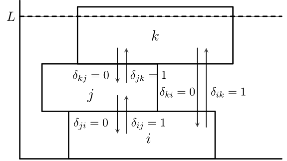
Fig. 4. Cover constraint on a non-ordered set of vessels violated.
