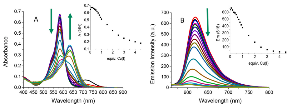
Fig. 7. A) Absorption and (B) emission ( \lambda_{\text{ex}} = 500 nm) changes observed for compound 1 (10 \mu\text{M} in DMSO:H 2 O 96:4) after the addition of increasing quantities of CuBr (0–4.5 equiv.) and their reaction profiles at 584 nm and 616 nm, respectively (insets).
