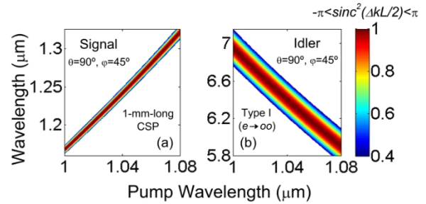
Fig. 1. Parametric gain bandwidth, -\pi < \text{sinc}^2(\Delta kL/2) < \pi , for type-I ( e \rightarrow \infty ) noncritical interaction, provided by a 1-mm-long CSP crystal for the (a) signal, and (b) idler, for pumping from 1 to 1.080 \mu\text{m} .
