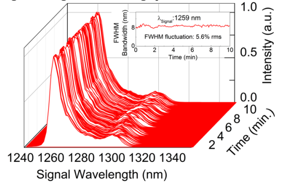
Fig. 7. Spectral stability of the signal extracted from the CSP OPO. Inset: Stability of the FWHM signal bandwidth.
