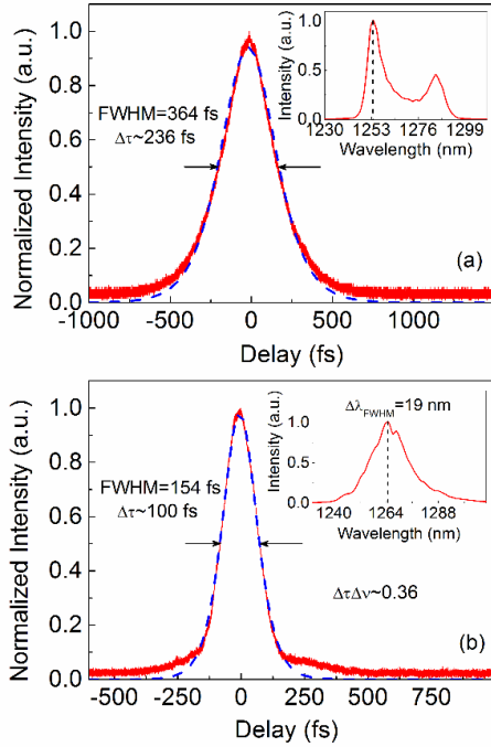
Fig. 8. Temporal profiles of the signal pulses extracted from the CSP femtosecond OPO (a) without, and (b) with dispersion compensation. Dashed blue traces are the \text{sech}^2 fit to the experimentally measured profiles. Inset: Corresponding signal spectra.
