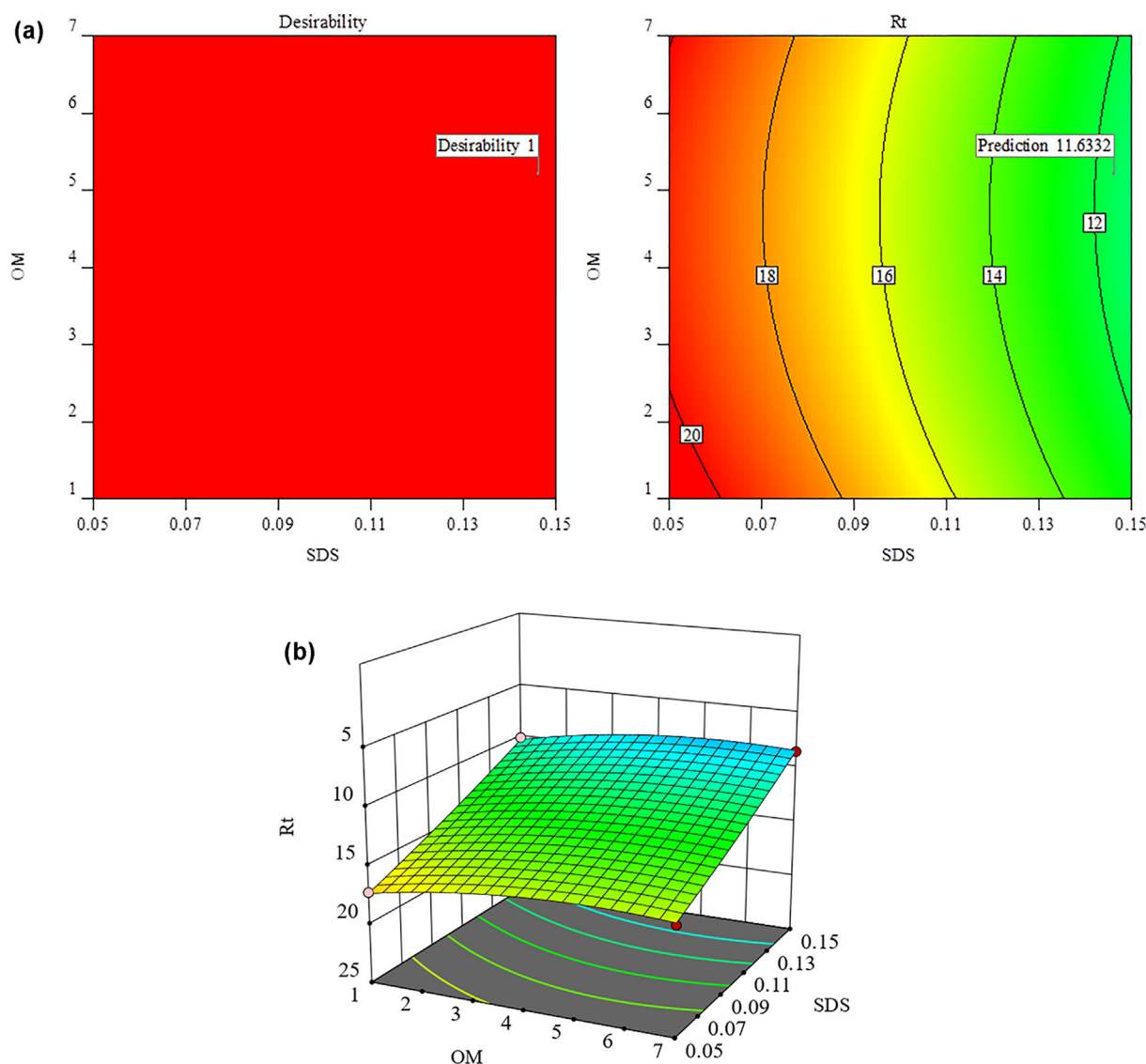
Fig. 5a. -b. Contour plots showing the influence of volume percentage of OM and SDS concentration on retention time of last eluted analyte.
