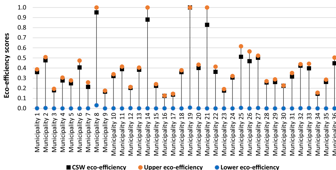
FIGURE 4 Upper, lower, and common set weights (CSW) eco-efficiency scores for the Chilean municipalities evaluated.
