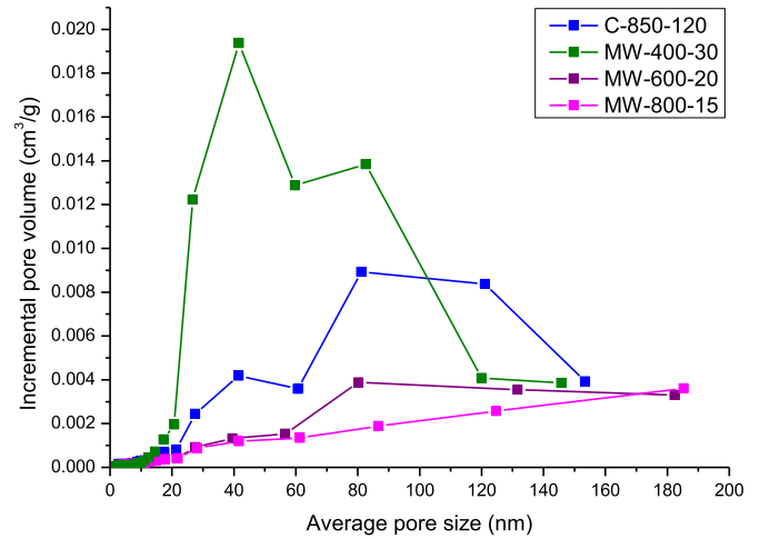
Fig. 5. Pore size distribution of conventional and microwave-treated samples using BJH (with Harkins-Jura correction) method.
