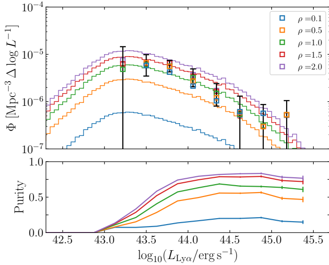
Fig. C.1. Effects of varying the sample purity on the estimated \text{Ly}\alpha LF. Top: Colored squares show different realizations of our \text{Ly}\alpha LF in the range z = 2.0 - 3.8 , obtained after scaling the number of true positives in the purity computation by a factor \rho = 0.1, 0.5, 1.0, 1.5, 2.0 . We also show the mock QSO LF for each \rho (solid lines). We show the uncertainties of the LF with \rho = 1 . The variation of the LF is inside the 1\sigma errors for all the shown values of \rho . Bottom: Estimated purity for the different values of \rho .
