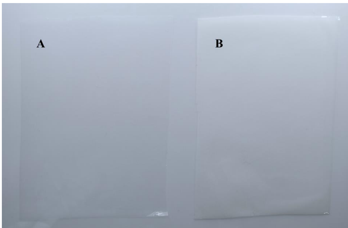
Figure 1. Film varnished with a coating thickness of 12 \mu\text{m} (a) and 24 \mu\text{m} (b). Coatings were prepared with 20% BN17-fermented whey (w/w) and 15% PVOH resin (w/w).
