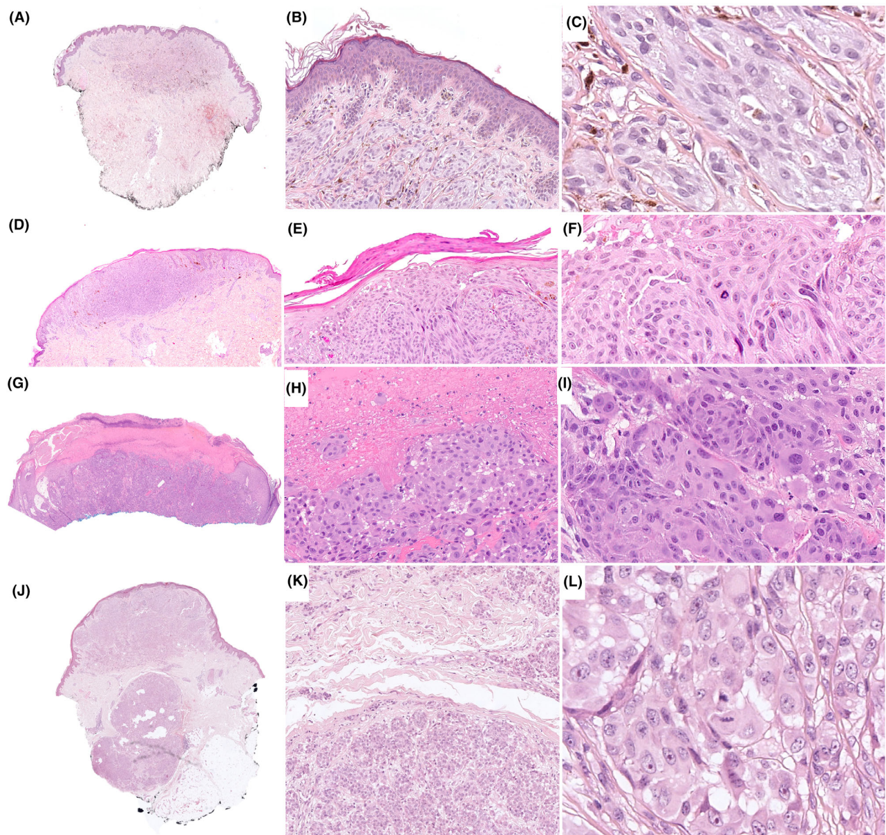
Figure 1. Spitzoid tumours: A–C. SN. D–F. Low-grade AS oidT with epidermal consumption and mitosis. G–I. High-grade AS oidT with ulceration and more prominent cellular atypia. J–L. (S oidM ) with penetrating expansile mass composed of atypical spitzoid melanocytes and deep mitosis.
