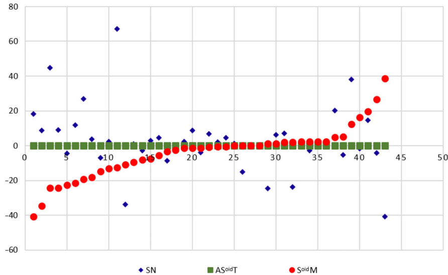
Figure 5. Dispersion map comparing the histological features between AS oidT , SN and S oidM .
