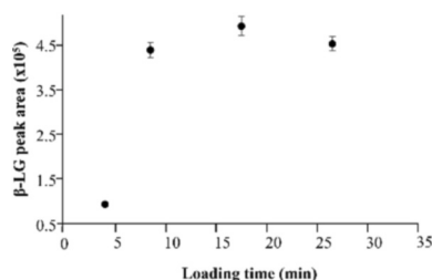
Fig. 2. Influence of the loading time at 930 mbar on the peak area of the detected β-LG (5 µg mL -1 β-LG standard solution in water) under the optimized elution and separation conditions.
