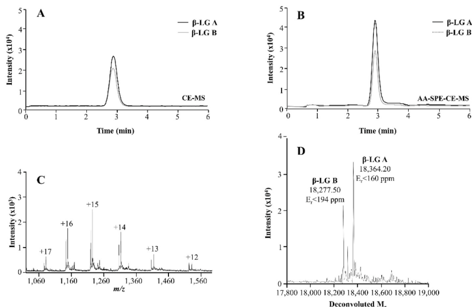
Fig. 1. (A) Extracted ion electropherograms (EIEs) for the CE-MS analysis of a 50 µg mL -1 β-LG standard solution; (B) EIEs for the AA-SPE-CE-MS analysis of a 1 µg mL -1 β-LG standard solution; (C) mass spectrum (by CE-MS) in the time window of the β-LG peak (ca. 3 min); and (D) deconvoluted mass spectrum (by CE-MS). ( E_r (ppm) = M_r experimental - M_r theoretical) / M_r theoretical \times 10^6 ).
