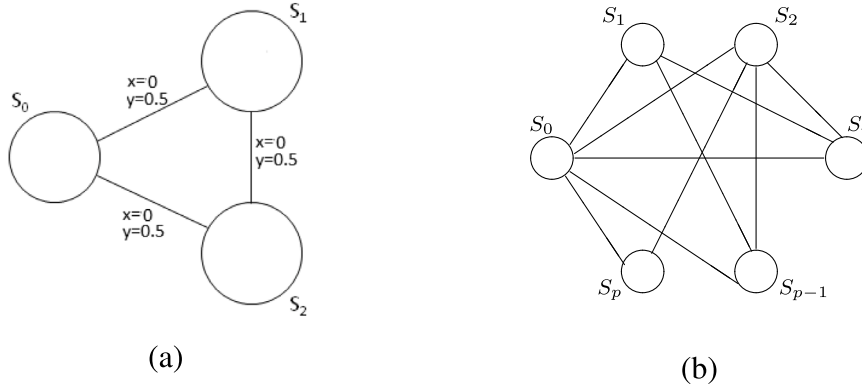
Fig. 5. p -connectivity inequalities.
