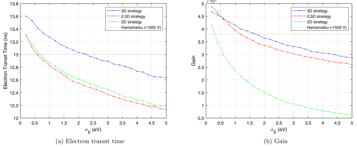
Fig. 5. PMT traits as a function of the parameter \sigma_E for the 3D, 2.5D and 2D strategies at a supply voltage U of -1500 V and k_\delta = 1 .
