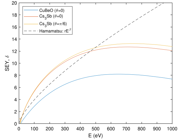
Fig. 3. Simulated SEY curves using the Modified Vaughan's model with \delta_{low} = 0.8, k_E = 1, k_\delta = 1, E_0 = 10 \text{ eV}, E_{max} = 650 \text{ eV}, \delta_{max} = 8.2 and \alpha = 0.95 for CuBeO and \delta_{low} = 0.8, k_E = 1, k_\delta = 1, E_0 = 9.15 \text{ eV}, E_{max} = 710 \text{ eV}, \delta_{max} = 12.7 and \alpha = 0.7377 for Cs 3 Sb. The parameters for the curve derived from the Hamamatsu datasheet are r = 0.1423, \beta = 0.7219 . The value of k_\delta will be fitted in Section 3.2.
