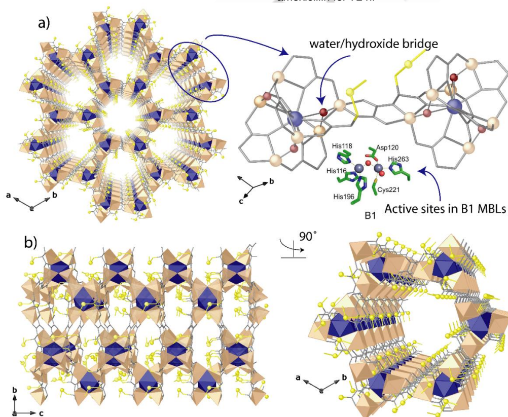
Figure 1. Crystal structure of 1 . a) Perspective views of 3D porous network of 1 along c crystallographic axis and a fragment (SBU) of 1 showing the dianionic bis(hydroxo)dizinc(II) building blocks. The inset shows a representative active-site \text{Zn}^{\text{II}} coordination geometry for B1 enzymes from Metallo- \beta -lactamases (MBLs), where \text{Zn}^{\text{II}} ions and water molecules/hydroxide ions are displayed as gray and red spheres, respectively. (b) Views of a fragment of 1 in the bc and ab planes. Zn, Ca and S atoms are represented by pale orange polyhedra, blue polyhedra, and yellow spheres, respectively, whereas the ligands(except sulfur) are depicted as gray sticks.
