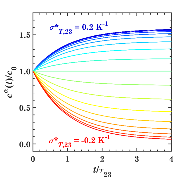
Figure 3. Simulated thermodiffusion of Na 2400 PSS. The concentration on the cold side ( \alpha ) changes when a temperature difference \Delta T = 20 K is applied. Depending on its effective Soret coefficient \sigma^*_{T,23} = 0.2 \text{ K}^{-1} \dots -0.2 \text{ K}^{-1} , the polyelectrolyte either accumulates at the cold side (thermophobic behavior, blue), or is depleted from the cold side (thermophilic behavior, red). Time is normalized with relaxation time \tau_{23} to help comparison, \omega = 0 .
