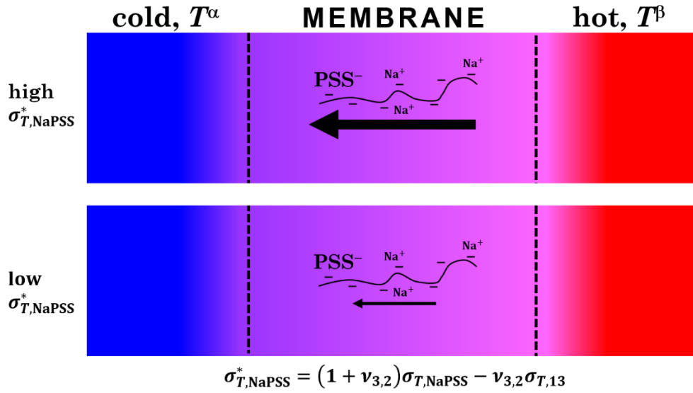
Figure 1. The polyelectrolyte (NaPSS) flows in a 1-1 supporting electrolyte (13) through a membrane that separates two chambers, \alpha and \beta , at temperatures T^\alpha and T^\beta and identical initial composition. The temperature difference induces a separation of NaPSS that is determined by its Soret coefficient \sigma_{T,\text{NaPSS}}^* in the mixture. This coefficient can be related to the Soret coefficients \sigma_{T,\text{NaPSS}} and \sigma_{T,13} of the polyelectrolyte and supporting electrolyte, respectively, and to the stoichiometric coefficient \nu_{3,2} of sodium in the polyelectrolyte.
