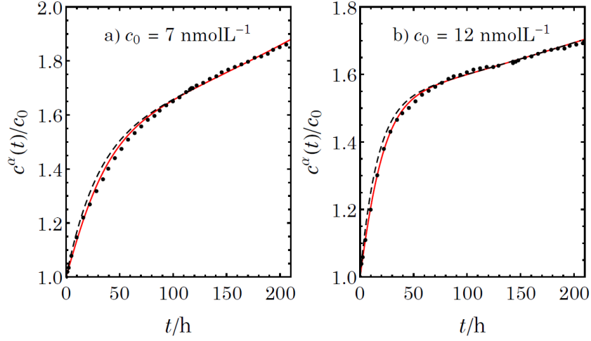
Figure 7. Since the supporting electrolyte diffuses faster than the polyelectrolyte, it seems reasonable for the sake of simplicity to assume that the former has reached the Soret equilibrium distribution while \text{Na}_{2400}\text{PSS} is still thermodiffusing. The symbols are experimental measurements of c_{23}^{\alpha}(t) . The solid lines show c_{23}^{\alpha}(t) from the exact numerical solution of the transport equations of the polyelectrolyte and the dashed lines from the approximate solution based on J_{13} \approx 0 (for the same parameter values). In all curves we have used \sigma_{T,13} = 2.3 \times 10^{-3} \text{K}^{-1} , \sigma_{T,23} = 3.8 \times 10^{-3} \text{K}^{-1} , \nu_{3,2} = 360 and V_0^{\alpha} = 5.8 \text{ mL} . Other parameter values are: a) \tau_{23} = 27.9 \text{ h} and \omega = 2.55 \times 10^{-7} \text{ s}^{-1} ; b) \tau_{23} = 15.6 \text{ h} and \omega = 1.45 \times 10^{-7} \text{ s}^{-1} . The values of \sigma_{T,23}^* can be calculated using eq 5.
