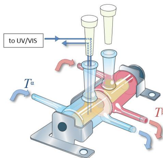
Figure 2. The Side-by-Side diffusion cell consists of two compartments of 3 mL, which can be set to different temperatures. Magnetic bars stir both sides. The total volume of the cold side ( \alpha ) when connected to a flow-through cuvette is 5 mL. Modified with permission from [34].
