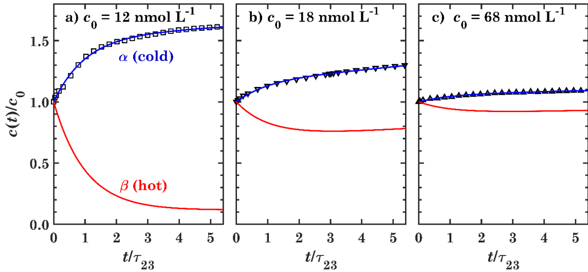
Figure 4. Thermodiffusion of \text{Na}_{2400}\text{PSS} in 0.1 \text{ mol L}^{-1} \text{ NaCl} at T_{\text{avg}} = 308 \text{ K} with \Delta T = 20 \text{ K} and a) c_0 = 12 \text{ nmol L}^{-1} ( 6 \text{ mg L}^{-1} ), b) c_0 = 18 \text{ nmol L}^{-1} ( 9 \text{ mg L}^{-1} ), and c) c_0 = 68 \text{ nmol L}^{-1} ( 34 \text{ mg L}^{-1} ). Symbols represent experimental values. Blue lines (cold \alpha -side) are best fits to eq 11 with the parameters shown in Table 1 and red lines represent eq 10 (hot \beta -side). The effect of a larger evaporation rate is noticeable in panel b), as the concentration in both chambers increase with time at larger times; note that the relaxation time \tau_{23} depends on c_0 .
