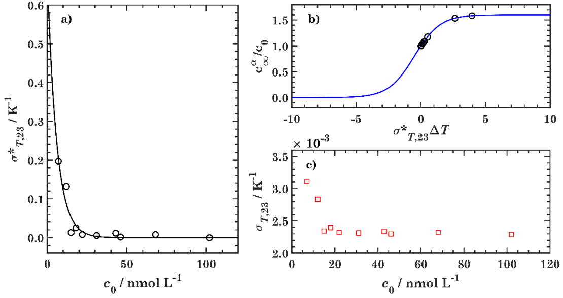
Figure 5. a) \sigma_{T,23}^* as a function of the initial concentration of the polyelectrolyte in 0.1 \text{ mol L}^{-1} NaCl (circles), black line an exponential fit to guide the eye. b) Theoretical steady-state concentration of the (cold) \alpha -side as a function of \sigma_{T,23}^* \Delta T (line) and the values (circles) calculated from \sigma_{T,23}^* in panel a. c) Estimated Soret coefficient for the polyelectrolyte in the absence of supporting electrolyte.
