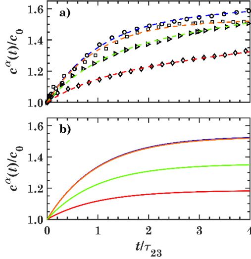
Figure 6. Thermodiffusion of \text{Na}_{2400}\text{PSS} ( c_{23} \approx 10 \text{ nmol L}^{-1} , T_{\text{avg}} = 308 \text{ K} , \Delta T = 20 \text{ K} ) in different 0.1 \text{ mol L}^{-1} supporting electrolytes. a) Experimental results are represented with symbols and dash lines are the best fits: NaCl (circles and blue), LiCl (squares and orange), \text{Na}_2\text{SO}_4 (triangles and green), and \text{NaClO}_4 (diamonds and red). b) Theoretical predictions without the effect of evaporation, i.e. \omega = 0 . Note that the difference between NaCl and LiCl is small and the curves practically overlap.
