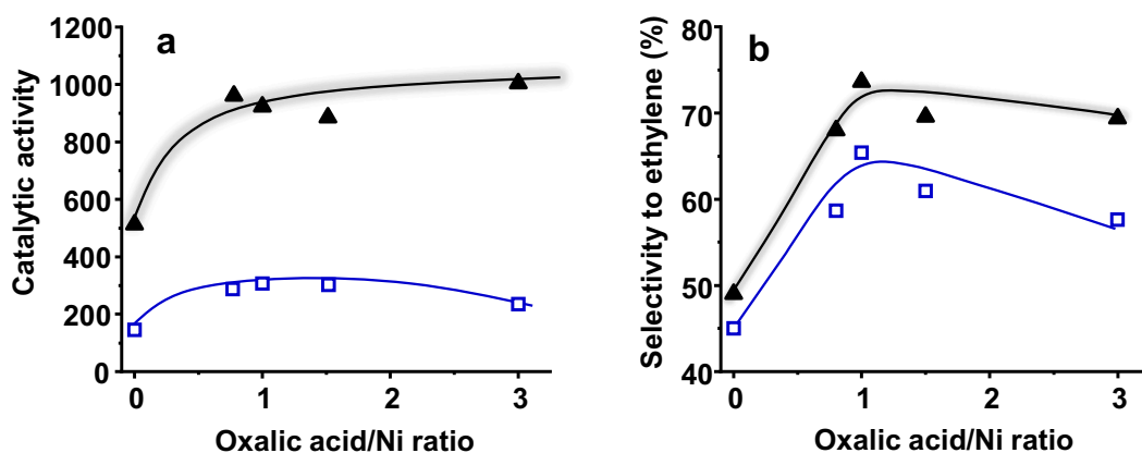
Fig. 1. Variation of: (a) the catalytic activity for ethane conversion, in \text{g}_{\text{C}_2\text{H}_6} \text{h}^{-1} \text{kg}_{\text{cat}}^{-1} ; and (b) the selectivity to ethylene at 300 °C and isoconversion conditions with the oxalic acid/Ni ratio in the synthesis gel. Symbols: catalysts calcined at 350 °C (▲) or 500 °C (◻) in air. Notes: Reaction conditions as in Table 2.
