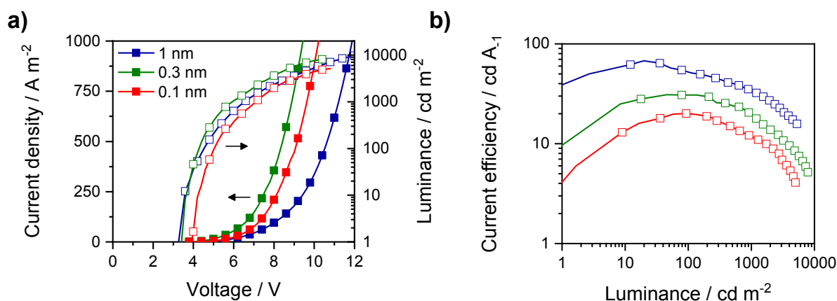
Figure 5. a) Current density–voltage–luminance ( J – V – L ) characteristics and b) current efficiency versus luminance for OLEDs with a m\text{-CsPbCl}_3 HTL and an ultrathin (1, 0.3 and 0.1 nm) vacuum-processed DMAC-TRZ active layer.
