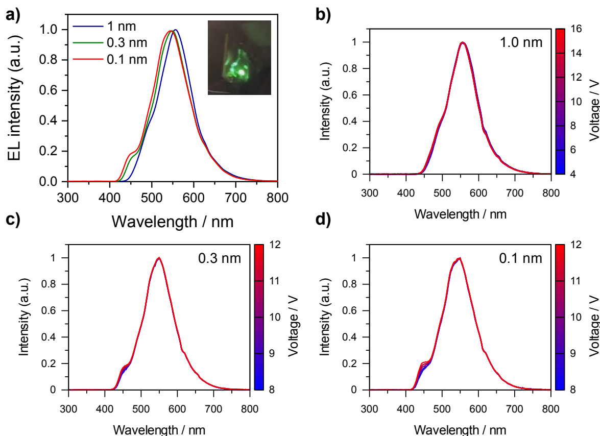
Figure 4. a) Electroluminescent spectra (10.0 V) for devices with different thicknesses (1, 0.3 and 0.1 nm) of the undoped DMAC-TRZ emissive layer (inset: photo of a working device with a 1 nm-thick emissive layer). b-d) electroluminescence spectrum versus voltage of devices with different DMAC-TRZ layer thicknesses: 1, 0.3 and 0.1 nm, respectively.
