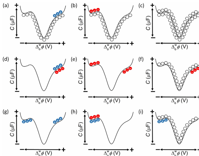
Figure 10. Schematic of the 9 possible distributions of the redox species in either side of the polarised L|L interface as a function of the applied \Delta\phi^w prior to the biphasic single-step IET reaction. A list of aqueous and organic redox species that could correspond to most of these panels is provided in Table S4.
