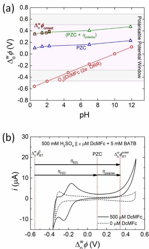
Figure 6. (a) A plot of \Delta_0^w \phi versus pH comparing the thermodynamically predicted \Delta_0^w \phi_{\text{onset}}^0 values as a function of pH for the biphasic 2e^- ORR with DcMFC as the organic electron donor (red circles, determined as described in Figure 1c), the PZC as a function of pH (blue triangles, determined from the differential capacitance measurements shown in Figure 6a and b) and the \Delta_0^w \phi_{\text{onset}}^0 values for the biphasic 2e^- ORR with DcMFC at acidic pH (purple squares, determined from the CVs shown in Figure 6d). The overpotential required to polarise the L|L interface sufficiently positive of the PZC to generate the [\text{H}^+ \dots \text{TB}^-] plateau region (as described in Figure 4) is assigned the value \eta_{\text{polarise}} = +0.240 V. The values of (\text{PZC} + \eta_{\text{polarise}}) (green triangles) overlap precisely with the \Delta_0^w \phi_{\text{onset}}^0 values at acidic pH. (b) As overlaid on the CV obtained at pH 0.55 in the presence of 500 μM DcMFC at a scan rate of 20 \text{ mV} \cdot \text{s}^{-1} (see Figure 2c), the overpotential to modulate the ion distribution in the back-to-back EDLs ( \eta_{\text{EDL}} ) to enable single-step IET at each pH for the biphasic 2e^- ORR with DcMFC, and thus \Delta_0^w \phi_{\text{onset}}^0 , is determined by an overpotential to reach the PZC ( \eta_{\text{PZC}} ) plus \eta_{\text{polarise}} .
