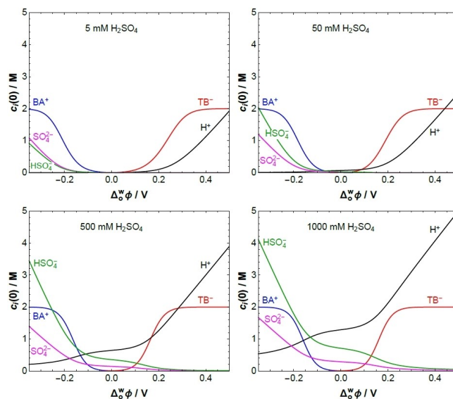
Figure 7. Interfacial concentrations vs. the applied interfacial Galvani potential difference \Delta_0^w \phi in Electrochemical Cell 1 (see Scheme 2a), 5 mM BATB (TFT) || y mM \text{H}_2\text{SO}_4 (aq), for y = 5, 50, 500 , and 1000 using a modified Verwey-Niessen model that accounts for the finite size of the organic phase ions. Their maximum concentration has been given the roughly estimated value of 2 M. At the positive end of the PPW, the proton concentration takes very similar values for y = 5, 50, 500 , and 1000; just like the sulfate ion and bisulfate ion concentration in the negative end of the PPW.
