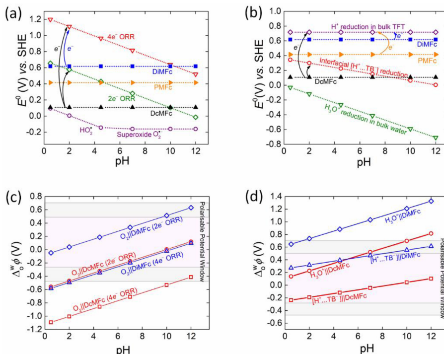
Figure 1. The thermodynamics of biphasic molecular oxygen ( \text{O}_2 ) reduction and biphasic proton reduction with organic solubilised electron donors at a polarised liquid|liquid (L|L) interface. (a) Plots of the standard redox potentials E^\circ vs. the standard hydrogen electrode (SHE) as a function of pH for (i) \text{O}_2 undergoing either a 2e^- or 4e^- \text{O}_2 reduction reaction (ORR) or forming perhydroxyl radicals ( \text{HO}_2^\bullet ) or superoxide radical anions ( \text{O}_2^{\bullet-} ) in a bulk aqueous solution, and (ii) the hydrophobic electron donors decamethylferrocene (DcMfc), pentamethylferrocene (PMFc) and dimethylferrocene (DiMfc) in the organic solvent \alpha,\alpha,\alpha -trifluorotoluene (TFT). (b) Plots of E^\circ vs. SHE as a function of pH for (i) the reduction of protons to molecular hydrogen ( \text{H}_2 ) for protons in an aqueous solution ( \text{H}_3\text{O}^+ ), organic TFT solution ( \text{H}^+ ), and accumulated in the EDL on the aqueous side of the L|L interface to compensate the charge of the organic electrolyte \text{TB}^- anions ( [\text{H}^+\cdots\text{TB}^-] ) in the mixed solvent region, and (ii) DcMfc, PMFc and DiMfc in TFT. (c) Plots of the standard Galvani interfacial electron transfer (IET) potential ( \Delta^\circ\phi_{\text{IET}}^w ) as a function of pH for the biphasic ORR ( 2e^- or 4e^- pathways) with DcMfc and DiMfc as the organic electron donors, respectively. For clarity the corresponding plot with PMFc is provided in Figure S2a. (d) Plots of \Delta^\circ\phi_{\text{IET}}^w as a function of pH for biphasic reduction of \text{H}_3\text{O}^+ and interfacial [\text{H}^+\cdots\text{TB}^-] with DcMfc and DiMfc as the organic electron donors, respectively. For clarity the corresponding plot with PMFc is provided in Figure S2b. In (c) and (d), the grey shaded areas of the Galvani polarisable potential window (PPW) represent applied interfacial Galvani potential differences ( \Delta^\circ\phi ) at the positive and negative extremes of the PPW that lead to significant changes in the polarity, viscosity, relative permittivity, and interfacial tension of the polarised L|L interface. The sources of electrochemical data and equations used to construct plots (a) and (b) are outlined in Table S1, plot (c) in Table S2 and plot (d) in Table S3.
