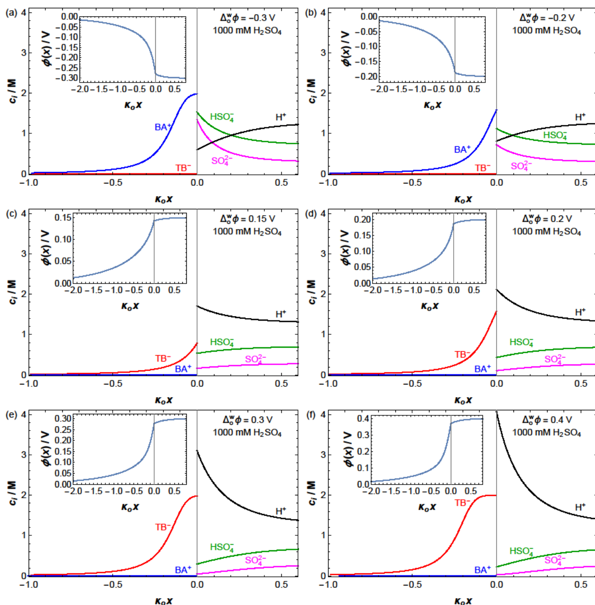
Figure S10. Ionic concentration profiles in Electrochemical Cell 1 (Scheme 2a), 5mM BATB (TFT) || 1000 mM H 2 SO 4 (aq), for applied \Delta_o^w \phi values of: (a) -0.3 V, (b) -0.2 V, (c) +0.15 V, (d) +0.2 V, (e) +0.3 V, and (f) +0.4 V. The maximum concentration of the organic ions due to their size has been given the roughly estimated value of 2 M. The L|L interface is located at x = 0 . Position x has been scaled with the reciprocal Debye length \kappa_o in phase o ( 1/\kappa_o = 1.489 nm). The insets show the corresponding electrical potential profiles.
