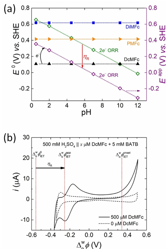
Figure 3. (a) Taking the intrinsic overpotential ( \eta_{\text{R}} ) of the biphasic 2\text{e}^- ORR at a polarised L|L interface into account, the apparent redox potential ( E^{\text{app}} , purple diamonds) required for \text{O}_2 to undergo a biphasic 2\text{e}^- ORR shifts negatively compared with E^0 (green diamonds). (b) In turn, as overlaid on the CV obtained at pH 0.55 in the presence of 500 \mu\text{M} DcMFC at a scan rate of 20 \text{mVs}^{-1} (shown previously in Figure 2b), the apparent Galvani IET potential ( \Delta_{\text{o}}^{\text{w}}\phi_{\text{IET}}^{\text{app}} ) shifts positively by \eta_{\text{R}} on the Galvani scale compared with \Delta_{\text{o}}^{\text{w}}\phi_{\text{IET}}^0 . The positive shift of \Delta_{\text{o}}^{\text{w}}\phi_{\text{IET}}^{\text{app}} is also shown in a plot of \Delta_{\text{o}}^{\text{w}}\phi versus pH for the biphasic 2\text{e}^- ORR with DcMFC in Figure S5. A further reason for the positive shift of \Delta_{\text{o}}^{\text{w}}\phi_{\text{IET}}^{\text{app}} compared to \Delta_{\text{o}}^{\text{w}}\phi_{\text{IET}}^0 is that the \Delta_{\text{o}}^{\text{w}}\phi_{\text{IET}}^0 values were calculated using the E^0 values for ORRs with aqueous \text{H}_3\text{O}^+ as the proton source, whereas more negative E^{\text{app}} values for ORRs involving interfacial [\text{H}^+ \dots \text{TB}^-] as the proton source may be more appropriate. Clearly, a major mismatch exists between the predicted value of \Delta_{\text{o}}^{\text{w}}\phi_{\text{IET}}^{\text{app}} and the experimentally observed onset interfacial Galvani potential difference ( \Delta_{\text{o}}^{\text{w}}\phi_{\text{IET}}^{\text{onset}} ) for the biphasic 2\text{e}^- ORR with DcMFC, which appears at a much more positive applied \Delta_{\text{o}}^{\text{w}}\phi .
