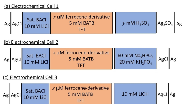
Scheme 2. Electrochemical cell configurations of the four-electrode electrochemical cells used. The ferrocene derivatives investigated were DcMFC, PMFc and DIMFc. In Electrochemical Cell 1, the \text{H}_2\text{SO}_4 concentration ( y mM) was adjusted to vary the pH from 0.36 to 2.26. The concentration of ferrocene derivative in the TFT organic phase is x \mu\text{M} . For blank experiments in their absence x=0 , and for experiments with a ferrocene derivative x=500 unless stated otherwise. In the organic reference solution, BACl is bis(triphenylphosphoranylidene)ammonium chloride, while BATB is the organic electrolyte salt bis(triphenylphosphoranylidene)ammonium tetrakis(pentafluorophenyl)borate. In this four-electrode configuration, the Pt electrode in the organic phase and Ag/AgCl electrode in the organic reference solutions (saturated BACl and 10 mM LiCl) were connected to the counter and reference terminals, respectively, while the Pt and Ag/AgCl (or Ag/Ag _2\text{SO}_4 ) electrodes in the aqueous phase were connected to the working and sensing terminals, respectively. All electrochemical experiments were carried out under aerobic, ambient conditions.
