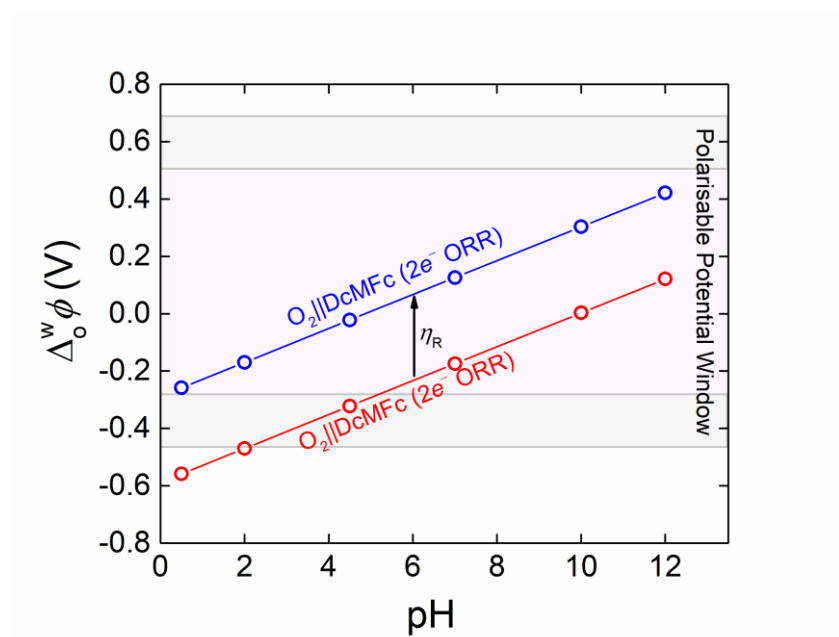
Figure S5. The apparent Galvani IET potential \Delta_0^w \phi_{\text{IET}}^{\text{app}} (blue circles) for the biphasic 2e^- ORR with DcMFC shifts positively by \eta_R on the Galvani scale compared with \Delta_0^w \phi_{\text{IET}}^0 (red circles) as shown in a plot of \Delta_0^w \phi versus pH.
