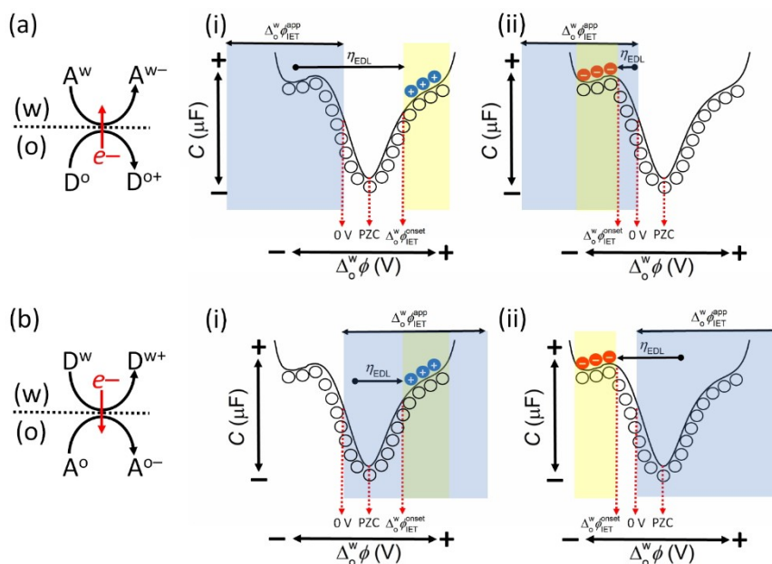
Figure 9. The distributions of the redox species on either side of the L|L interface as a function of the applied \Delta\phi^w are depicted by overlaying cationic (blue circle), anionic (red circle) or neutral (hollow circle) symbols on a differential capacitance measurement with features typically observed at the polarised L|L interface (as described in detail in Figures 4 and 8). A symbol above the line represents an aqueous redox species A^w or D^w , whereas a symbol below the line represents an organic redox species A^o or D^o . Such schemes allow ease of visualisation of the relationships between \Delta\phi^w_{\text{onset}} , \Delta\phi^w_{\text{app}} , and \eta_{\text{EDL}} , which are dependent on whether electrons flow from (a) the organic to aqueous phase or (b) the aqueous to organic phase, and whether \Delta\phi^w_{\text{onset}} is (i) positive or (ii) negative of 0 V on the Galvani scale. \Delta\phi^w_{\text{onset}} in turn is dependent on the nature of the ion distributions in the back-to-back EDLs as a function of the applied \Delta\phi^w . For example, if the redox species A^w or D^w is cationic then \Delta\phi^w_{\text{onset}} will be in the potential range positive of the PZC [yellow shaded areas in (a)(i) and (b)(ii)], while if A^w or D^w is anionic then \Delta\phi^w_{\text{onset}} will be in the potential range negative of the PZC [yellow shaded areas in (a)(ii) and (b)(i)]. The flow of electrons from the organic to the aqueous phase is spontaneous when \Delta\phi^w_{\text{onset}} < 0 V on the Galvani scale [blue shaded areas in (a)(i) and (a)(ii)]. The flow of electrons from the aqueous to the organic phase is spontaneous when \Delta\phi^w_{\text{onset}} > 0 V [blue shaded areas in (b)(i) and (b)(ii)]. \Delta\phi^w_{\text{app}} can have a value outside the PPW.
