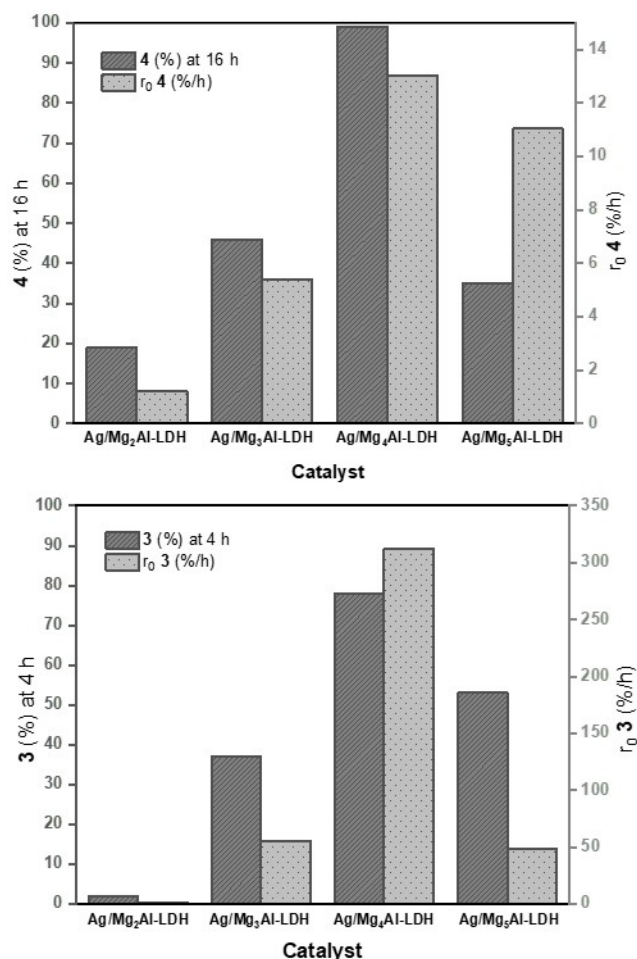
Figure 2. Initial reaction rates of 3 and 4 formation ( r_0 ) expressed as [yield (%)/h] and yield of 3 and 4 at a defined reaction time for (up) \alpha -alkylation of phenylacetonitrile 1 with benzyl alcohol 2 (3 equiv.) at 140 °C and (bottom) condensation step between phenylacetonitrile 1 and benzaldehyde 5 (3 equiv.) at 110 °C in the presence of different [\text{Ag}/\text{Mg}_x\text{Al-LDH}] materials. For detailed reaction conditions, see SI. Yield of products 3 and 4 were calculated by GC using hexadecane as internal standard. Initial rate ( r_0 ) is the slope of the linear equation: [yield of 3 (%)] = r_0 \times t (h) or [yield of 4 (%)] = r_0 \times t (h)] defined at initial reaction times and expressed as [ r_0 3 (%/h)] or [ r_0 4 (%/h)].
