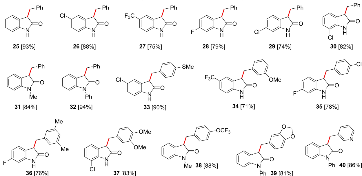
Scheme 3. Synthesis of \alpha -functionalized (A) nitriles and (B) 2-oxindoles through [Ag/Mg 4 Al-LDH]-catalyzed \alpha -alkylations using primary alcohols via BH strategy. [a] Standard reaction conditions: nitrile or oxindole (0.125 mmol), alcohol (0.375 mmol, 3 equiv.), freshly reduced [Ag/Mg 4 Al-LDH] catalyst (at 130 °C, 2 h, heating ramp of 0.5 °C/min) with a silver content of 0.5 wt% (134 mg, 5 mol% Ag), mesitylene (1.5 mL) at 140 °C under N 2 during 24 h. Yields of isolated products are given between brackets. [b] Run with 2.5 mol% Ag (67 mg of catalyst). [c] Run with alcohol (0.625 mmol, 5 equiv.) for 48 h. [d] Run during 48 h.
