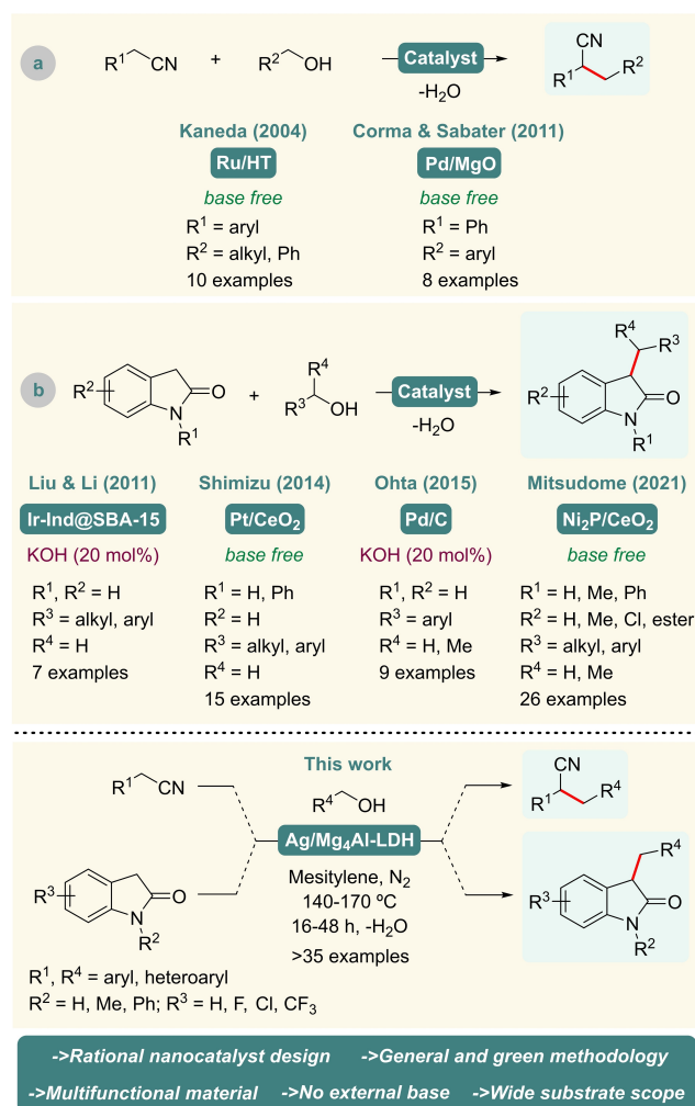
Scheme 1. Top: Heterogeneously catalyzed reported examples for \alpha -alkylation of nitriles (a) or oxindoles (b) using alcohols via borrowing hydrogen methodology. Bottom: [Ag/Mg 4 Al-LDH]-catalyzed \alpha -alkylation of nitriles and oxindoles with alcohols reported in this work. HT = hydrotalcite support with a molecular formula [\text{Mg}_6\text{Al}_2(\text{OH})_{16}\text{CO}_3 \cdot 4\text{H}_2\text{O}] . Ind = indene.
