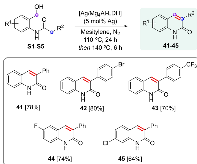
Scheme 4. [Ag/Mg 4 Al-LDH]-catalyzed one-pot synthesis of 3-arylquinolin-2(1H)-ones 41–45 from the intramolecular \alpha -alkylation of 2-phenylacetamide groups with primary alcohols. Standard reaction conditions: N -[2-(hydroxymethyl)phenyl]-2-phenylacetamide S1–S5 (0.125 mmol), freshly reduced [Ag/Mg 4 Al-LDH] catalyst with a silver content of 0.5 wt % (134 mg, 5 mol % Ag), mesitylene (2 mL), under N 2 at 110 °C during 24 h and then at 140 °C over 6 h. Yields of isolated products are given between brackets.
