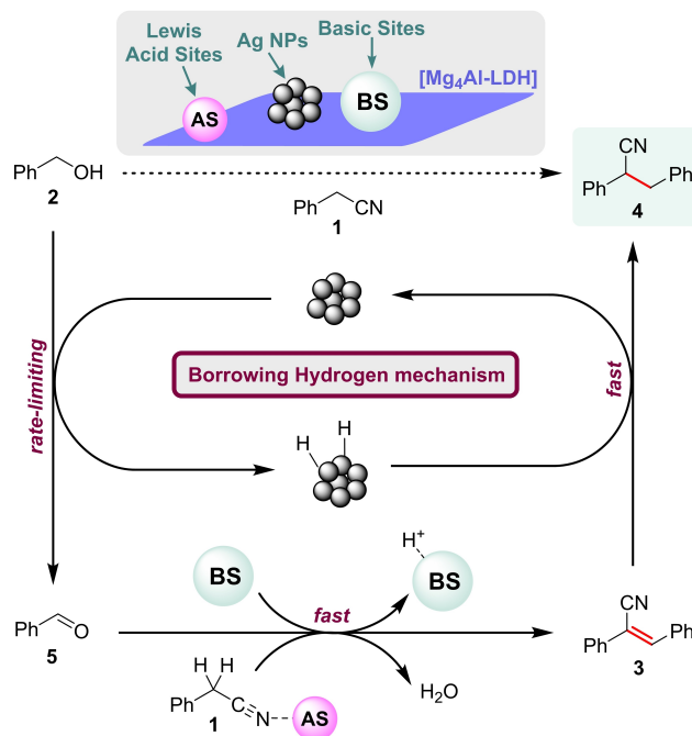
Scheme 2. Plausible reaction mechanism for the \alpha -alkylation of phenylacetonitrile 1 with benzyl alcohol 2 in the presence of [\text{Ag}/\text{Mg}_4\text{Al-LDH}] nanocatalyst.
