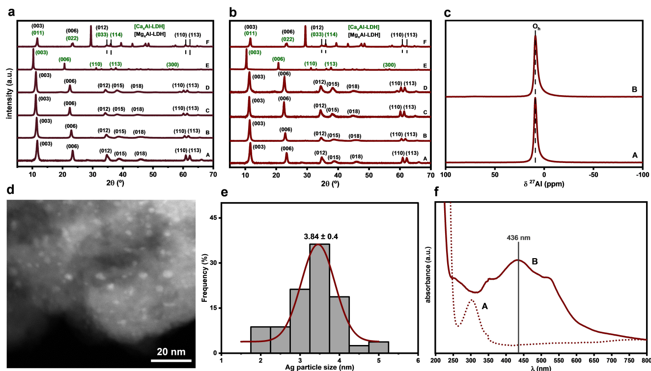
Figure 1. Selected characterization data of [LDH] and [Ag/LDH] nanomaterials: a) XRPD patterns of freshly prepared LDH solid supports: (A) [Mg 2 Al-LDH], (B) [Mg 3 Al-LDH], (C) [Mg 4 Al-LDH]; (D) [Mg 5 Al-LDH]; (E) [Ca 2 Al-LDH]; (F) [Ca 2 Mg 2 Al-LDH]; b) XRPD patterns of freshly reduced LDH-supported silver materials at 130 °C and 0.5 °C/min: (A) [Ag/Mg 2 Al-LDH], (B) [Ag/Mg 3 Al-LDH], (C) [Ag/Mg 4 Al-LDH], (D) [Ag/Mg 5 Al-LDH], (E) [Ag/Ca 2 Al-LDH] and (F) [Ag/Ca 2 Mg 2 Al-LDH]; c) 27 Al MAS NMR spectra of freshly prepared (A) [Mg 4 Al-LDH] support and (B) [Ag/Mg 4 Al-LDH] material freshly reduced at 130 °C and 0.5 °C/min; d) HAADF-HRSTEM image of freshly reduced [Ag/Mg 4 Al-LDH] material at 130 °C and 0.5 °C/min; e) Particle size histogram of the HAADF-HRSTEM study of [Ag/Mg 4 Al-LDH] material reduced at 130 °C and 0.5 °C/min; f) Diffuse Reflectance UV-vis spectra of (A) [Mg 4 Al-LDH] support, (B) freshly reduced [Ag/Mg 4 Al-LDH] material at 130 °C and 0.5 °C/min.
