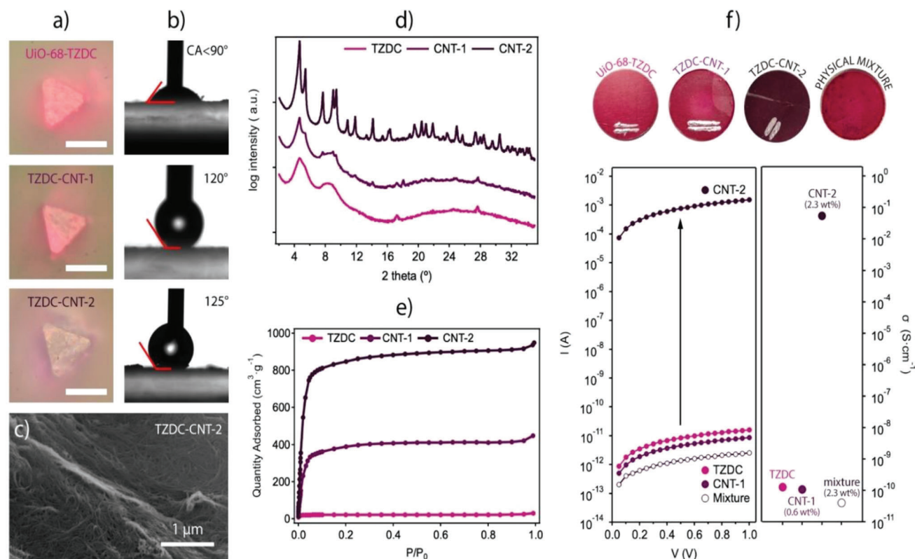
Figure 4. a) Crystals of UiO-68-TZDC, TZDC-CNT-1, and TZDC-CNT-2. Scale bars correspond to 15 μm. b) Contact angle measurements confirming their hydrophobicity after CNT linkage. c) SEM image of the crystal surface of CNT-2. d) PXRD and e) N 2 isotherms after incubation in water for 24 h showing the effect of the nanotube layer in protecting the crystals from chemical degradation and structural collapse. f) Pellets used for the transport measurements (top). I–V plots (left) and conductivity values (right) at room temperature.
