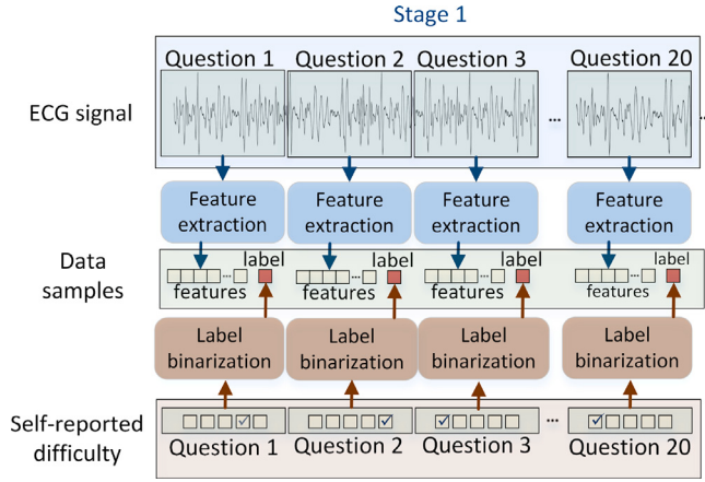
Fig. 1. Construction of the D_{pre} dataset used to estimate difficulty from the ECG signals.
