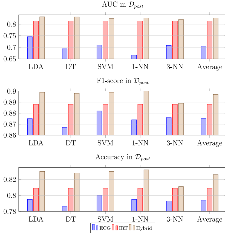
Fig. 5. Comparison of difficulty estimation using ECG signals, IRT and the hybrid approach, for the \mathcal{D}_{post} dataset, according to the classifier used. Average results across all classifiers are also reported on the right-most bars. The evaluation includes the three different measures considered in the study, namely AUC, F1-scores, and accuracy. The top row displays the AUC results, the middle row showcases F1-scores, and the bottom row illustrates accuracy results.
