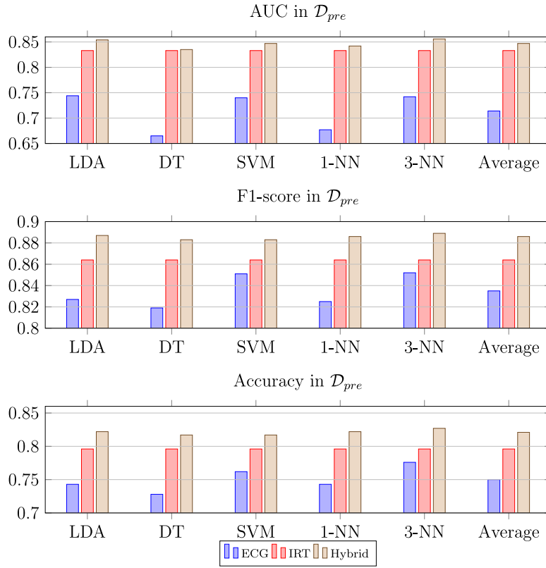
Fig. 4. Comparison of difficulty estimation using ECG signals, IRT and the hybrid approach, for the \mathcal{D}_{pre} dataset, according to the classifier used. Average results across all classifiers are also reported on the right-most bars. The evaluation includes the three different measures considered in the study, namely AUC, F1-scores, and accuracy. The top row displays the AUC results, the middle row showcases F1-scores, and the bottom row illustrates accuracy results.
