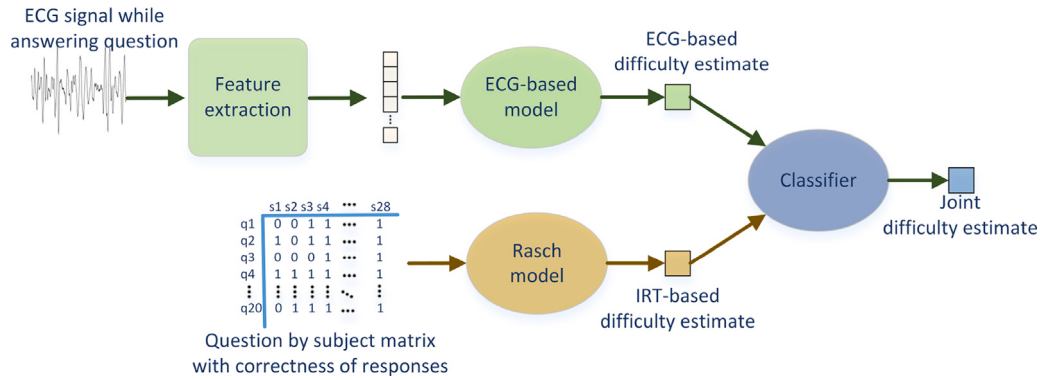
Fig. 2. Fusion of difficulty scores estimated by using ECG signals and IRT.
