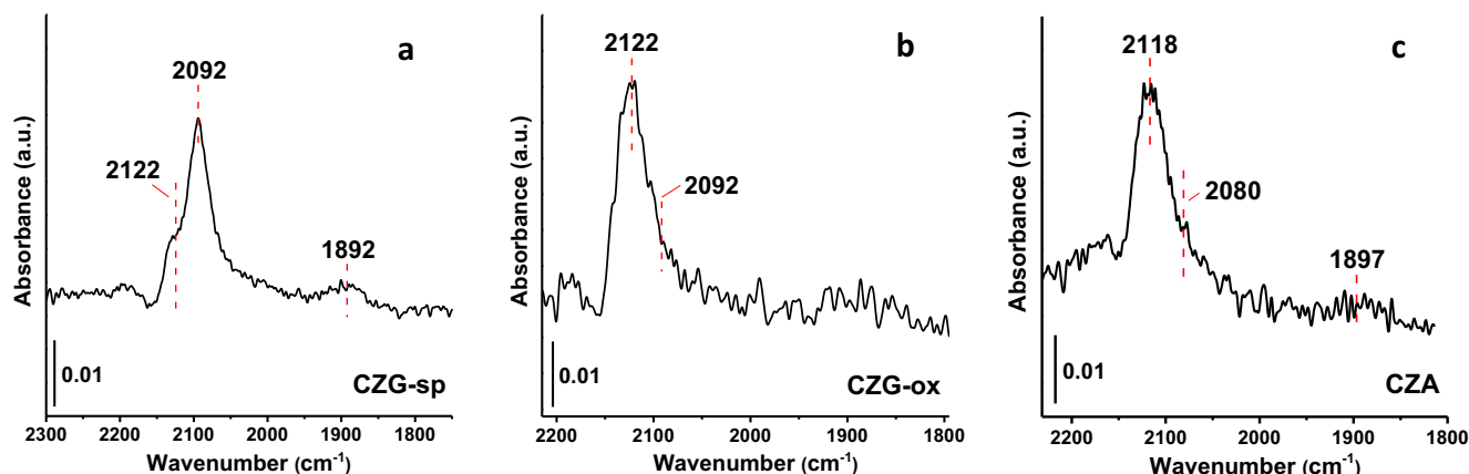
Fig. 7. IR spectra of CO adsorbed at -50^{\circ}\text{C} on in situ reduced CZG-sp, CZG-ox and CZA samples.
