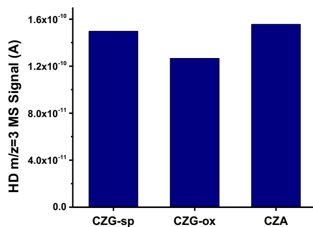
Fig. 8. \text{H}_2 - \text{D}_2 isotopic exchange results for CZG and CZA samples at 90^{\circ}\text{C} .
