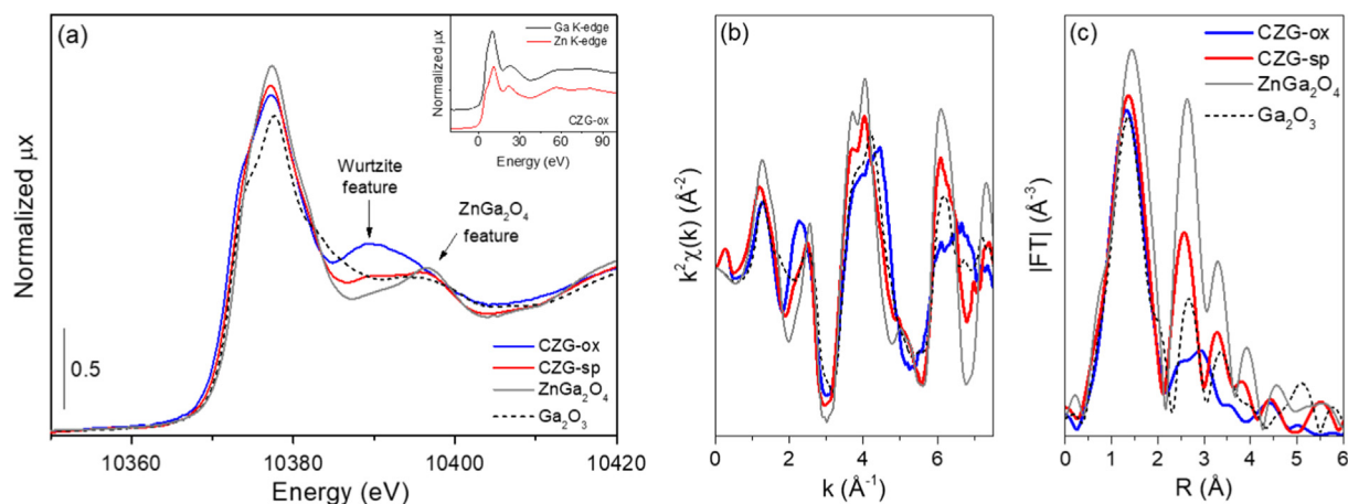
Fig. 1. Normalized XANES spectra at Ga K-edge (a), phase-uncorrected, k^2 -weighted \chi(k) functions (b) and EXAFS spectra (c) of CZG catalysts and Ga-based references. Inset: comparison of CZG-ox sample measured at Ga and Zn K-edges showing the similarity in XANES features, attributed in literature to wurtzite-type structures [31,32].
