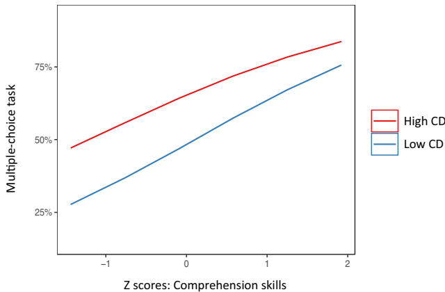
Fig. 1. Predicted probabilities for the multiple-choice task. The upper curve shows high contextual diversity (CD), and the lower curve shows low CD.
