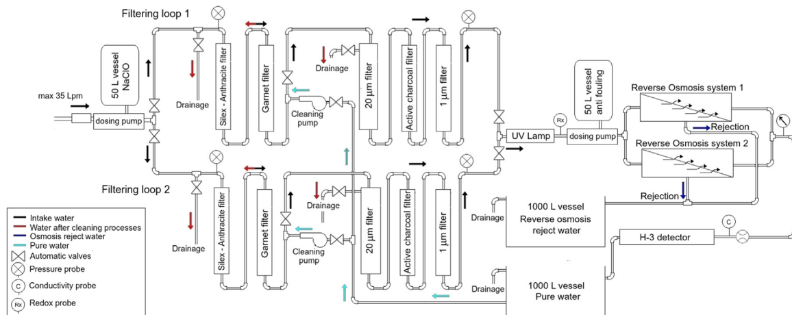
Fig. 3. Scheme of the water treatment plant installed in RAREx water monitoring station in the Tagus River.
